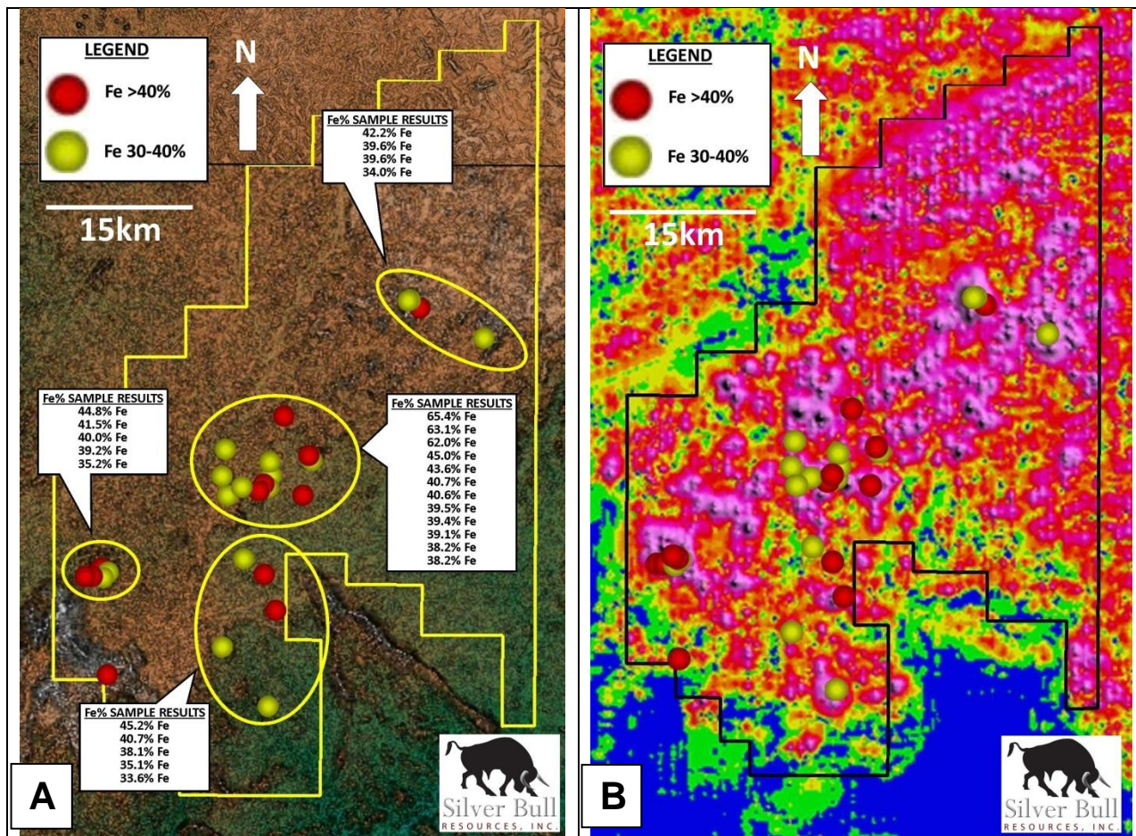
Figure 2. Results from the sampling program >30% Fe shown in map "A" from the regional reconnaissance sampling program on the Mitzi license. The same samples set against the regional magnetic map shown in Map "B" on the Mitzi license. There are over 70km of magnetic highs in the area which correspond to topographic highs.
