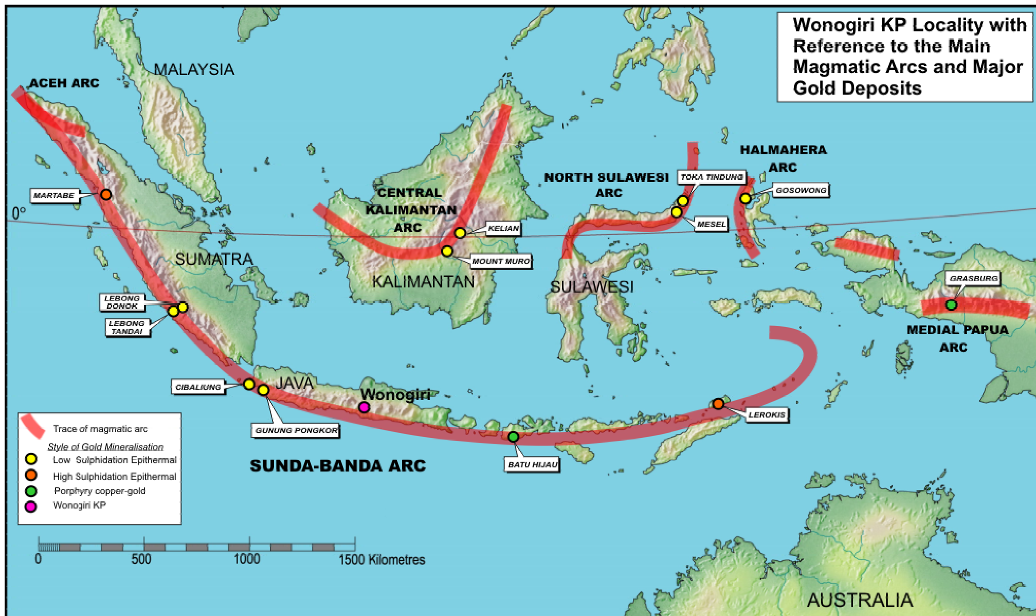
Figure 1: Wonogiri KP Locality Plan with reference to major magmatic arcs and gold deposits.
