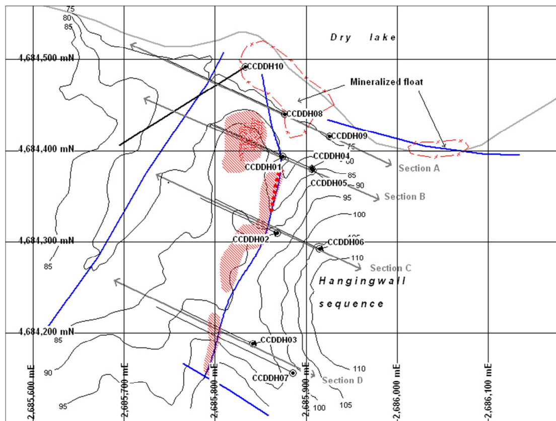
Figure 2. Cerro Cubilete, drill-hole and drill section location plan. Selected fault traces are shown in blue, outcropping mineralization in red. Topographic contours are in meters.
