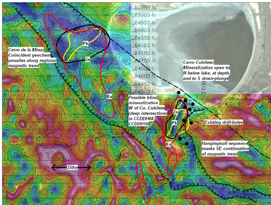
Figure 5. Cerro Cubilete and Cerro de la Mina. Rock chip geochemical anomalies are superimposed on a ground magnetic (tilt derivative) image, illustrating the NW-trending magnetic feature which appears to constrain mineralization at both Cerro Cubilete and Cerro de la Mina. Underlying Quickbird satellite image shows the ephemeral lake to the north of the prospect.
