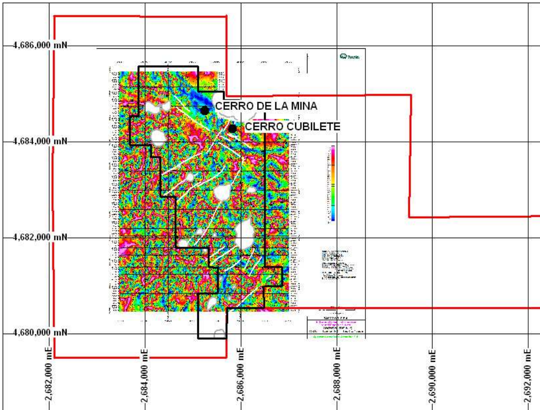
Figure 2. Corina and Mercia tenements, showing extent of geological mapping (black outline) and ground magnetic (tilt derivative) image. Mapped faults are shown as white lines, white areas are small dry lakes, red outline is property boundary. Gridlines are 2 km apart.
