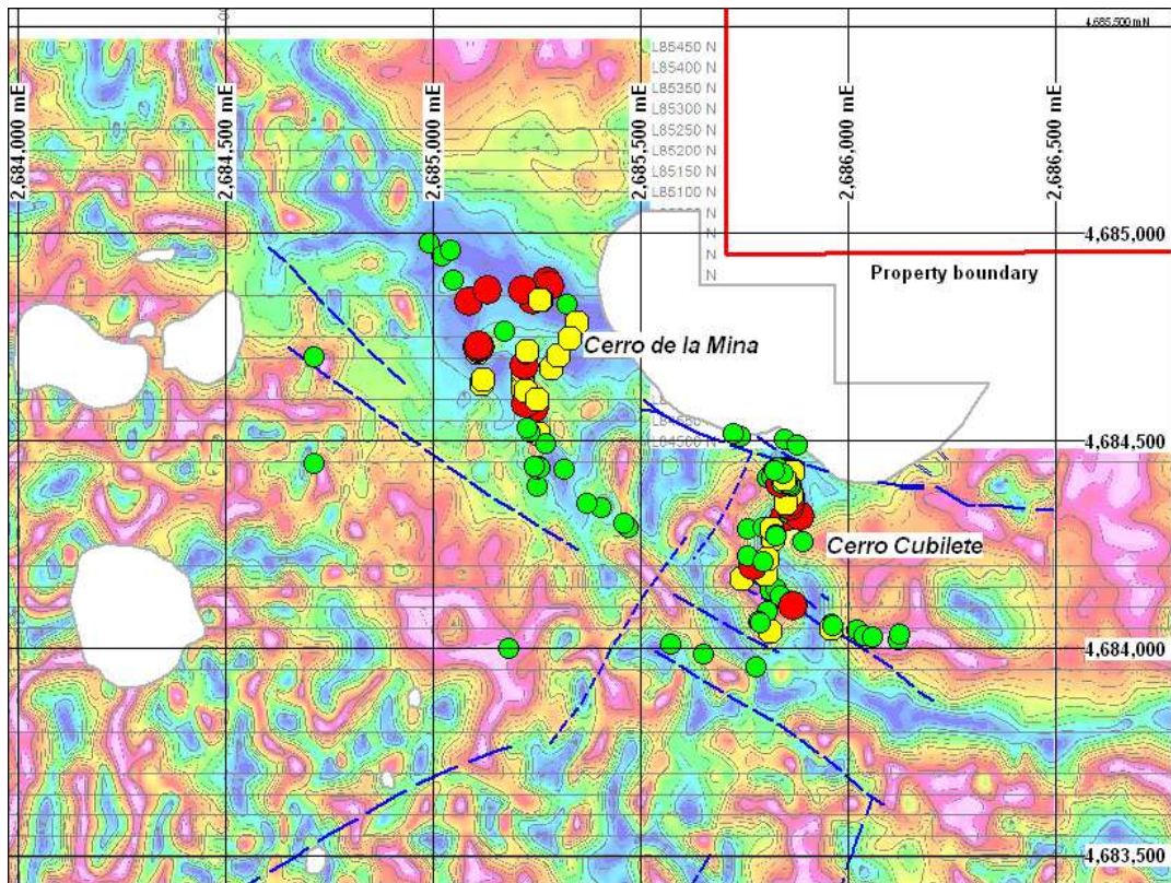
Figure 4. Cerro Cubilete-Cerro de la Mina area. Part of ground magnetic (tilt derivative) image with superimposed As thematic map (red = >72, yellow = 28-72, green = <28 ppm As). Blue lines are mapped faults. Gridlines are 500m apart.
