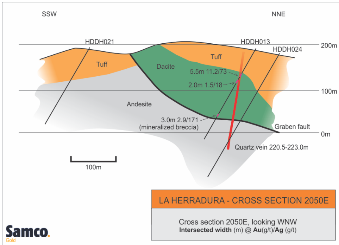
Figure 4. Cross section 2050E, looking WNW, showing drill-holes, interpreted geology, and intersections (width in m, g/t Au/g/t Ag). See Figure 2 for section line
