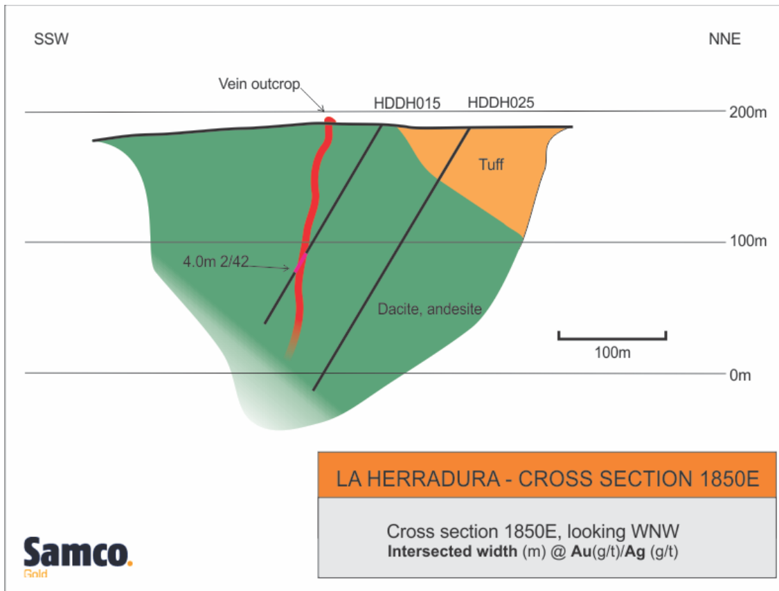
Figure 5. Cross section, 1850E, looking WNW, showing drill-holes, interpreted geology, and intersection (width in m, g/t Au/g/t Ag. See Figure 2 for section line
