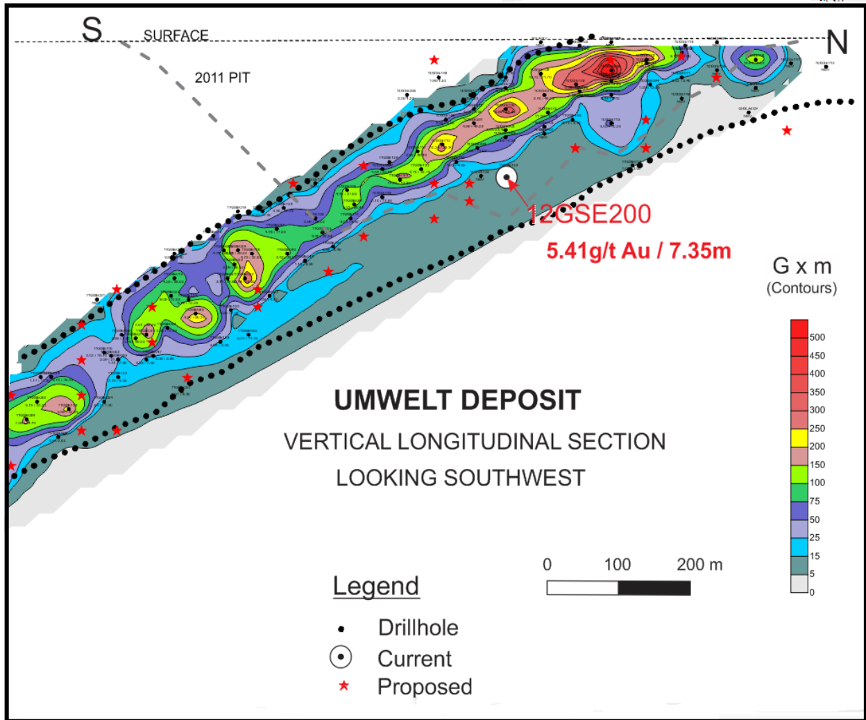
Figure 3: Umwelt Main Longitudinal Section
