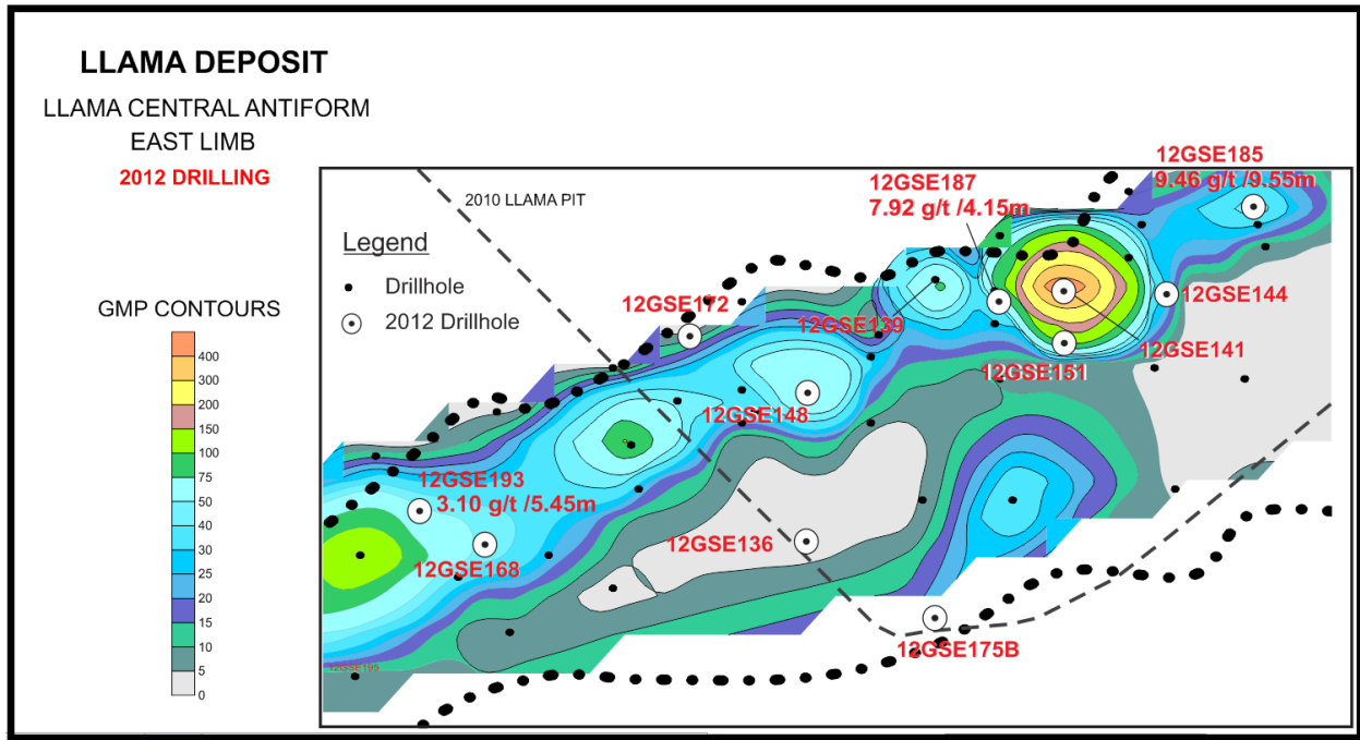
Figure 1: Llama East Limb Longitudinal Section
