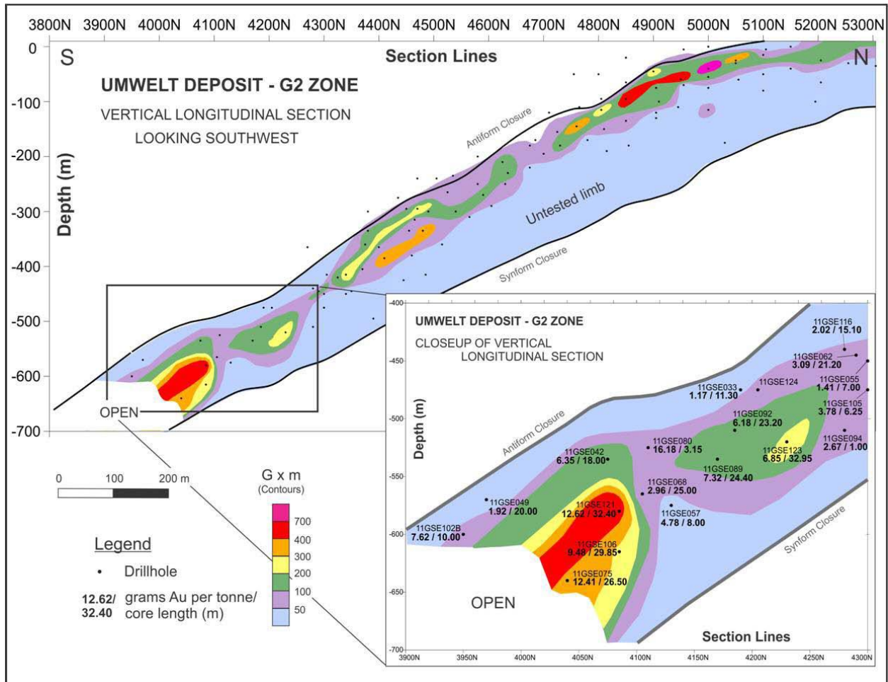
Figure 2: Umwelt Deposit grade x thickness longitudinal section.
