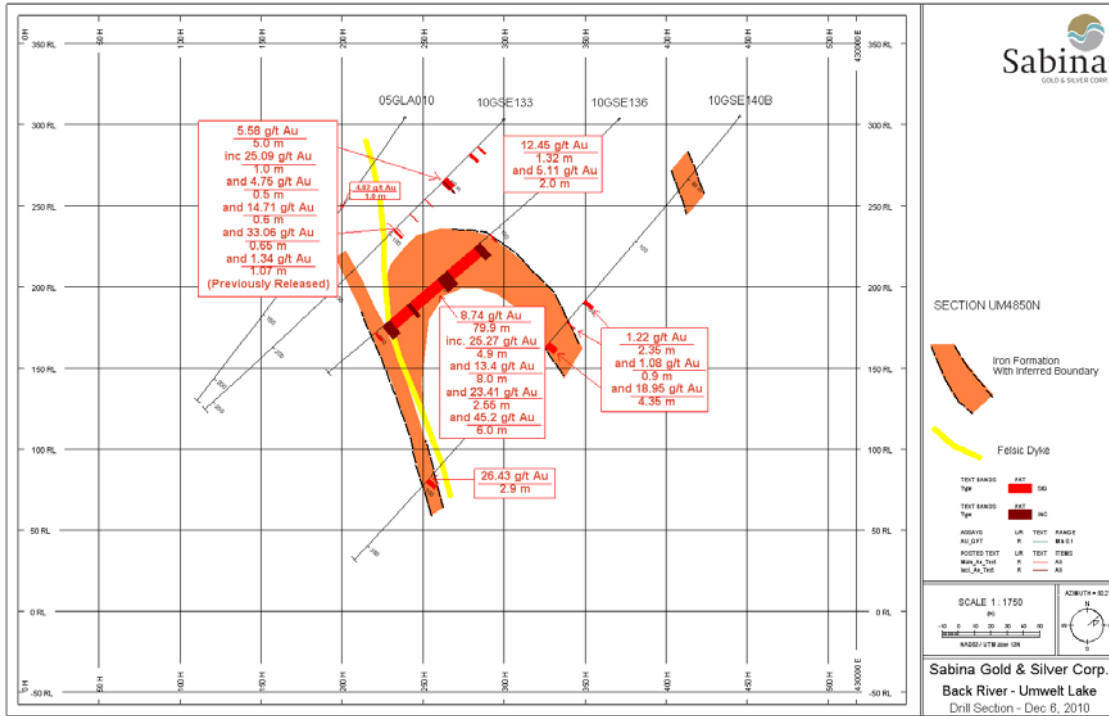
Figure 3: Umwelt Section 4850N.
