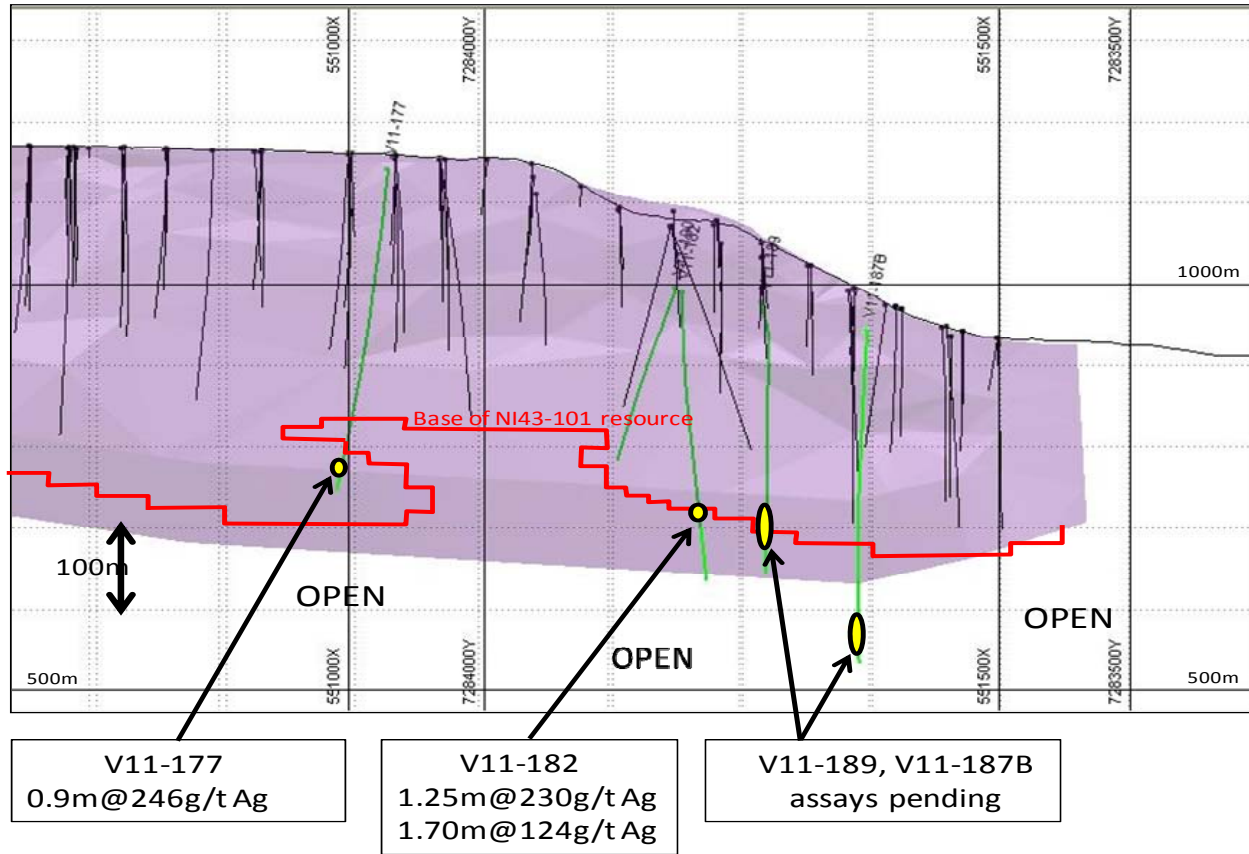
Figure 3: Longitudinal Section of Southern Portion of Central Zone, showing new drill Intersections extending NI 43-101 compliant mineral resource blocks below the February 2011 estimate
