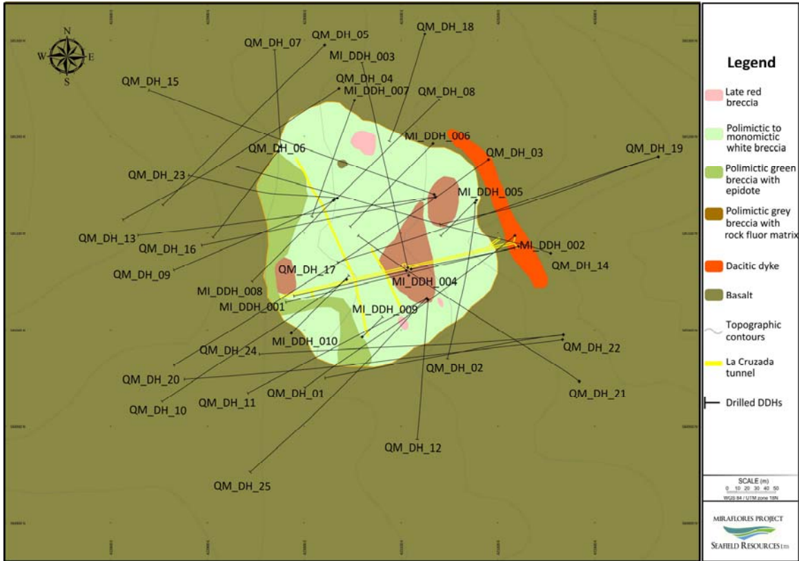
Map 1 – Geology and Drill Locations
