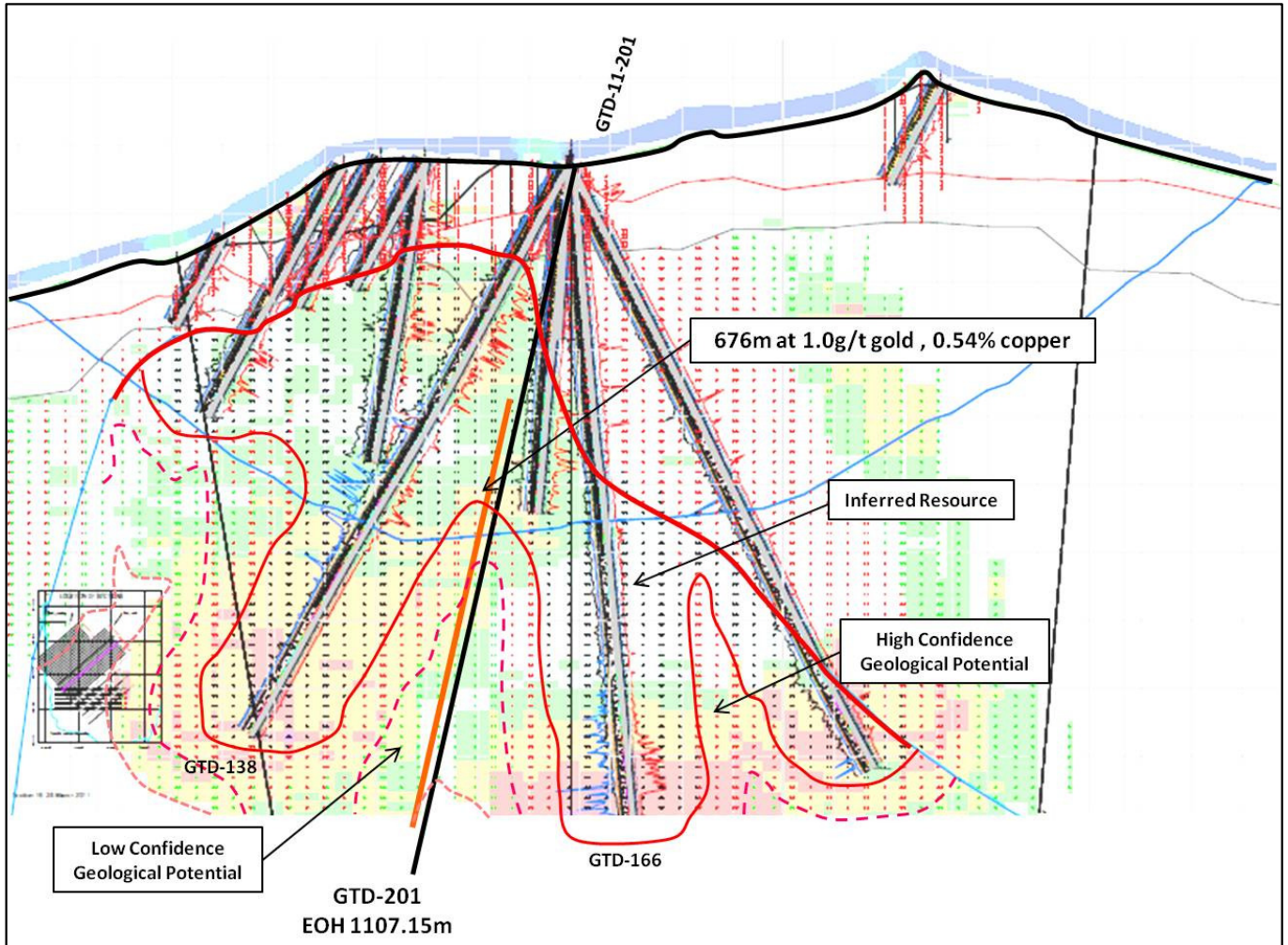
Section through drill holes GTD-201, 138 and 166.
