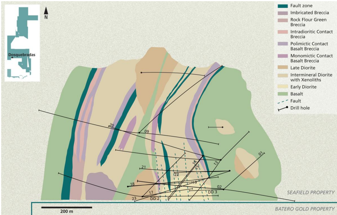
Figure 1 - Drill Plan View of Dosquebradas:
