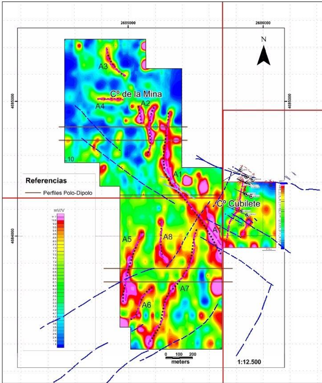
Figure 2. Area of the gradient array IP survey, showing numbered chargeability anomalies A1 to A8, Cerro Cubilete drill-holes, and inferred faults from previous geological mapping. Pole dipole lines are shown as pairs of EW lines crossing the surveyed area.
