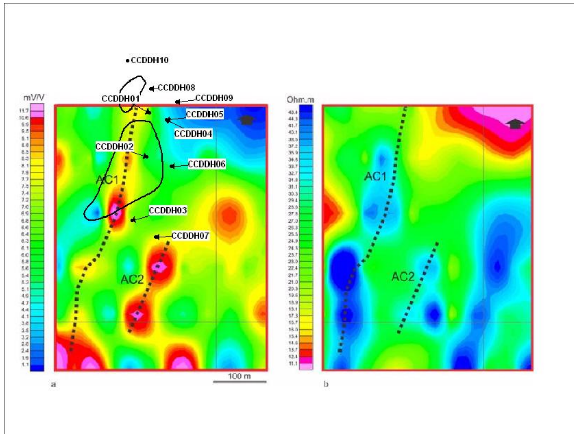
Figure 6. Cerro Cubilete gradient array chargeability (a) and resistivity (b) images. Numbered anomalies are described in the text. The chargeability image also shows drill-holes and rock chip Pb anomalies
