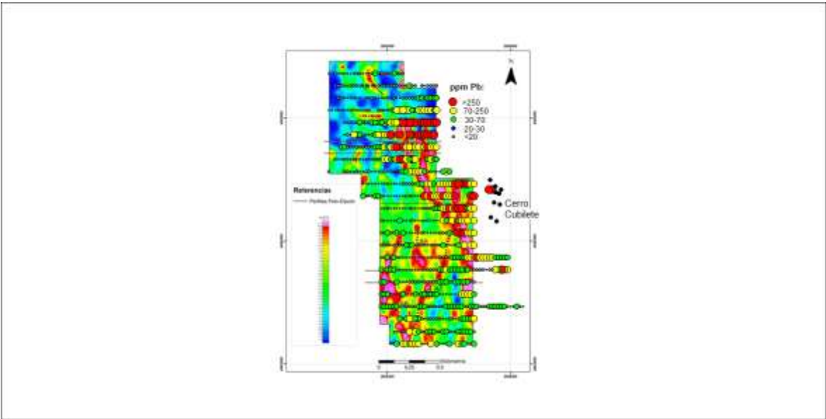
Figure 2. Corina lag sample grid showing distribution of Pb values, other features as per Figure 1
