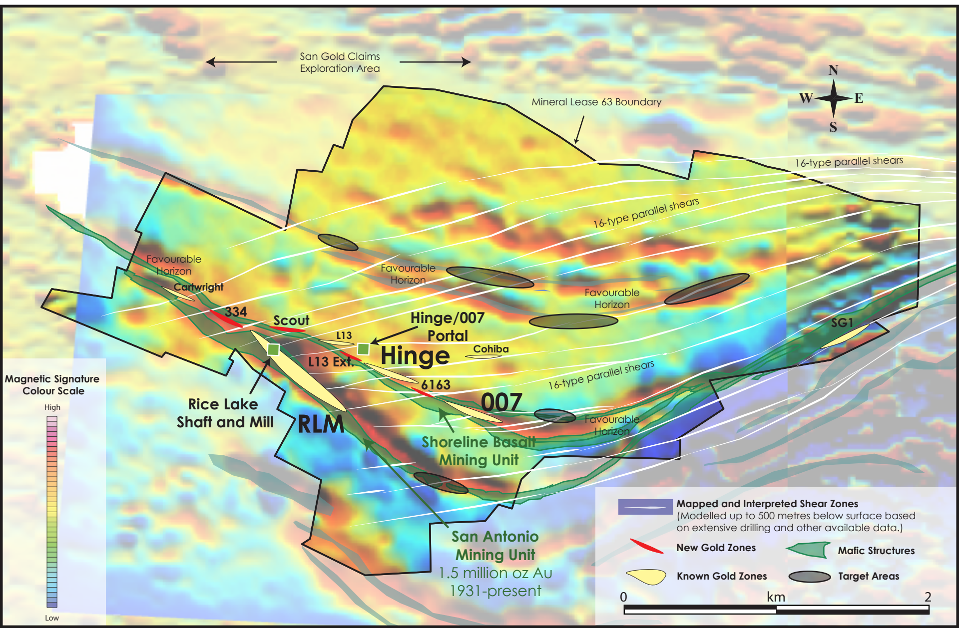
Figure 1: Plan View of Magnetic Survey with Interpreted Regional Shear Zones
