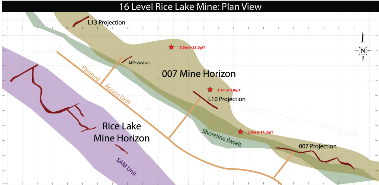
Figure 3 16 Level Plan View Showing Nearby Pierce Points and Spatial Relationships between Rice Lake Mine, Shoreline Basalt, and L10, L13 and 007 Zones.
