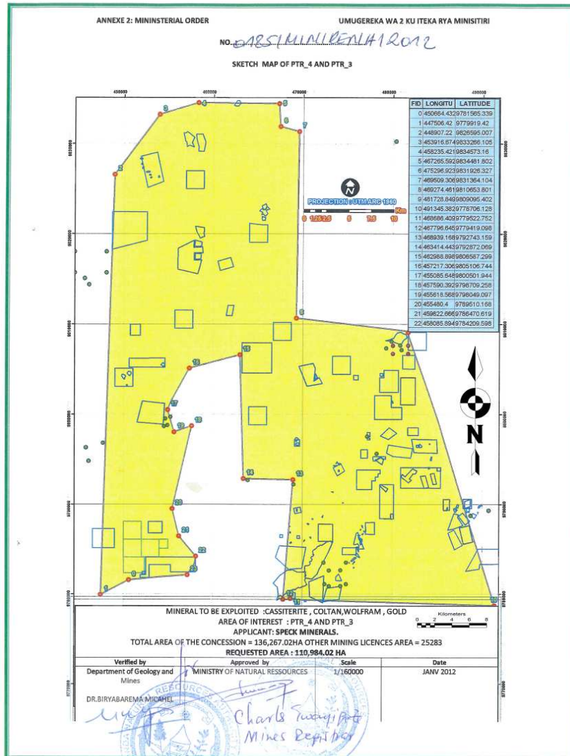
Figure 2. Documented artisanal licences in the Rurembo Project Area
