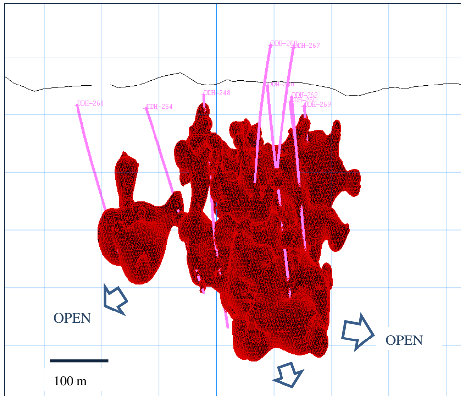
Figure 2: Interpreted Volume of the Cortaderas Breccia Mineralized Body
