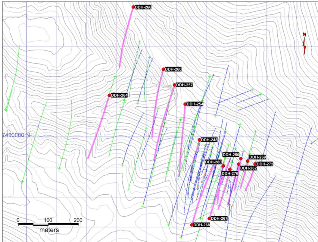
Figure 1: Plan map of the Cortaderas Target Area on the Pirquitas Mine Property
