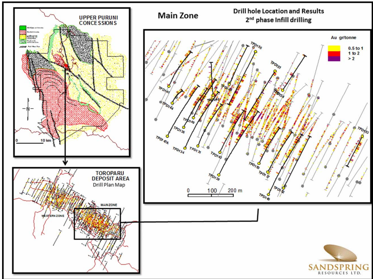
Figure 2: Toroparu location, Drill Plan Map, and detailed location of holes TPD 143-155 relative to NI 43-101 Mineral Resource Contour disclosed in March 21, 2011 Press Release
