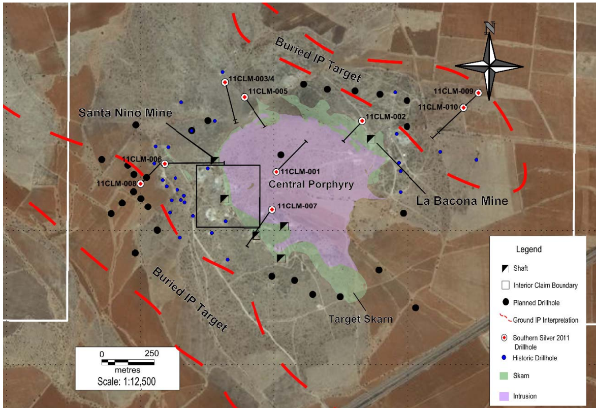
Figure 1: Plan view of the area of historic mining at the Cerro Las Minitas Project showing the distribution of current, historic and planned drill holes. Gravel covered geophysical targets, outlined in red, highlight the exploration potential of the project.
