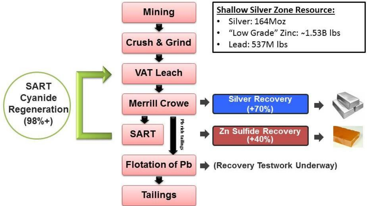
Figure 2. Mining flow sheet for silver mineralization at Sierra Mojada
