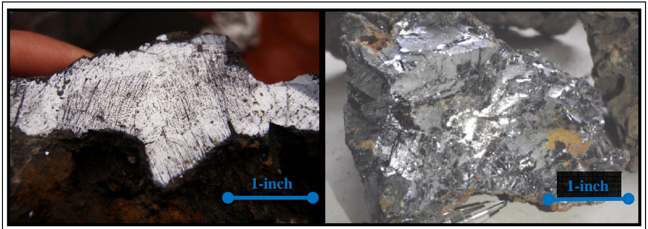
Figure 3: Massive argentiferous galena mineralization from Fault-2.
