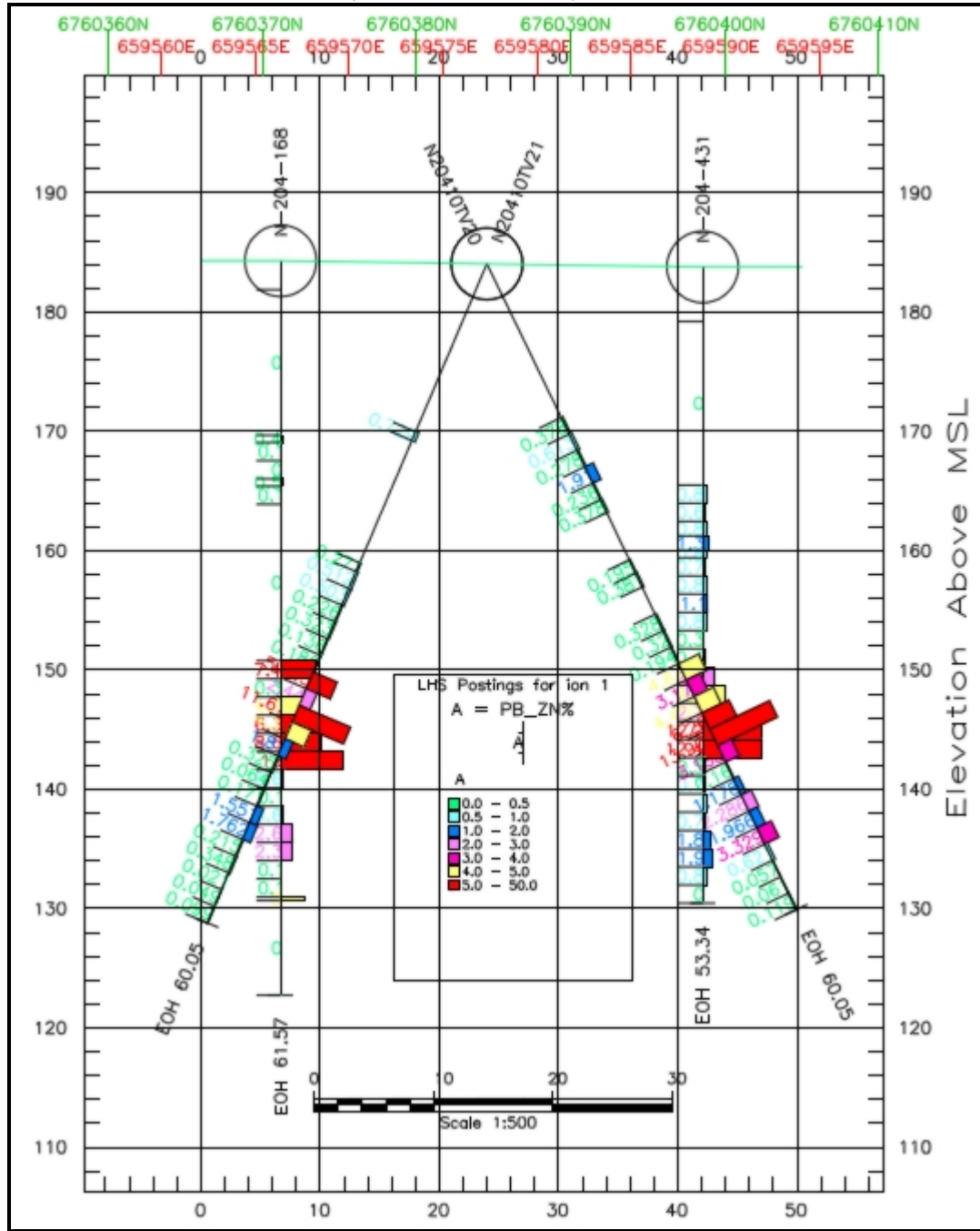
NE-SW Cross-Section Looking NW through Holes N204-10-TV20 and TV21 (All units in meters)
