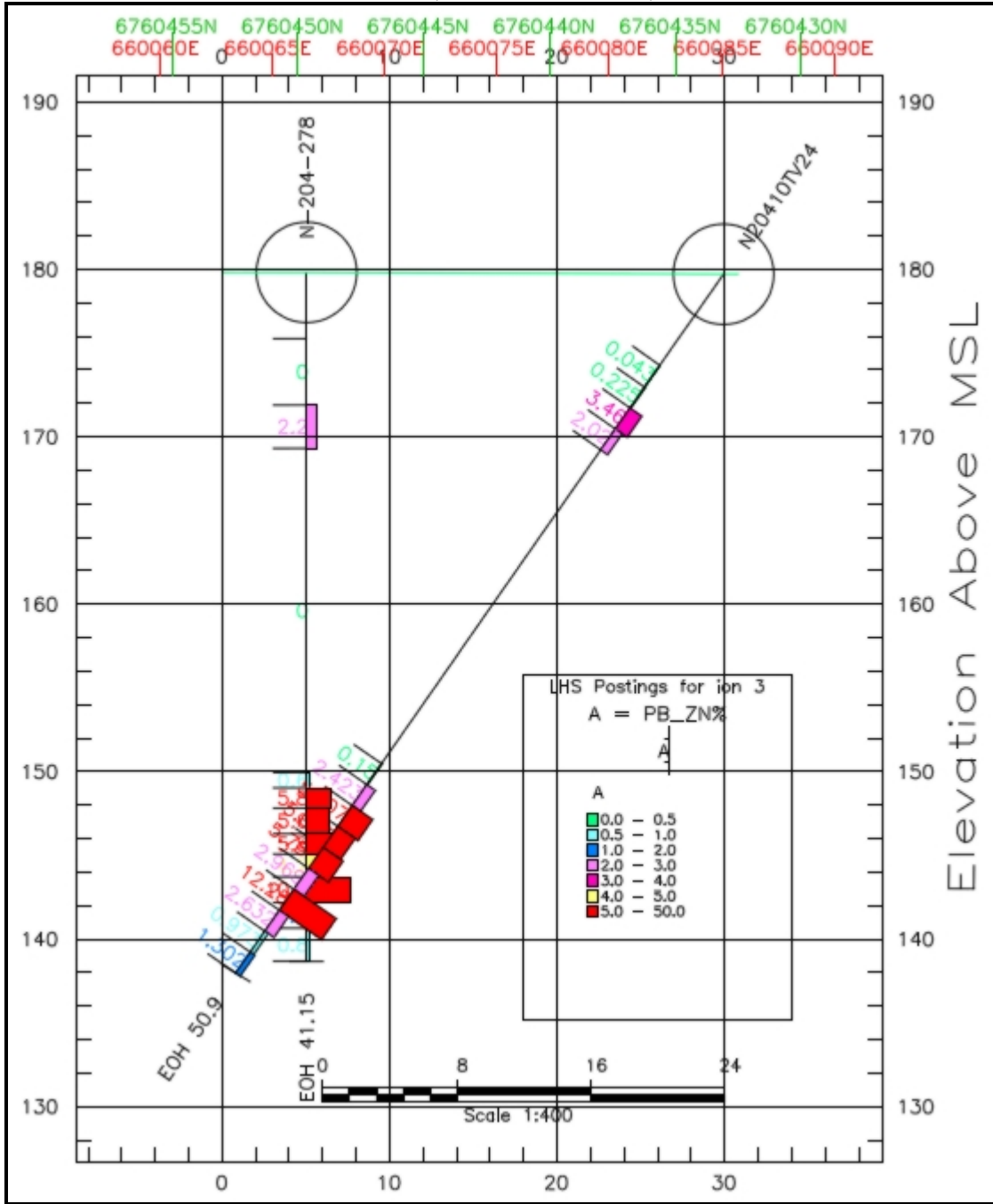
NW-SE Cross-Section Looking SW through Hole N204-10-TV24 (All units in meters)
