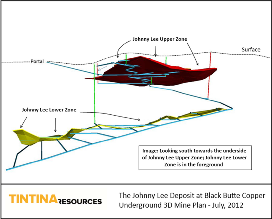
Figure 3 Black Butte Copper Project Underground 3-D Mine Plan Meagher County, MT, USA
