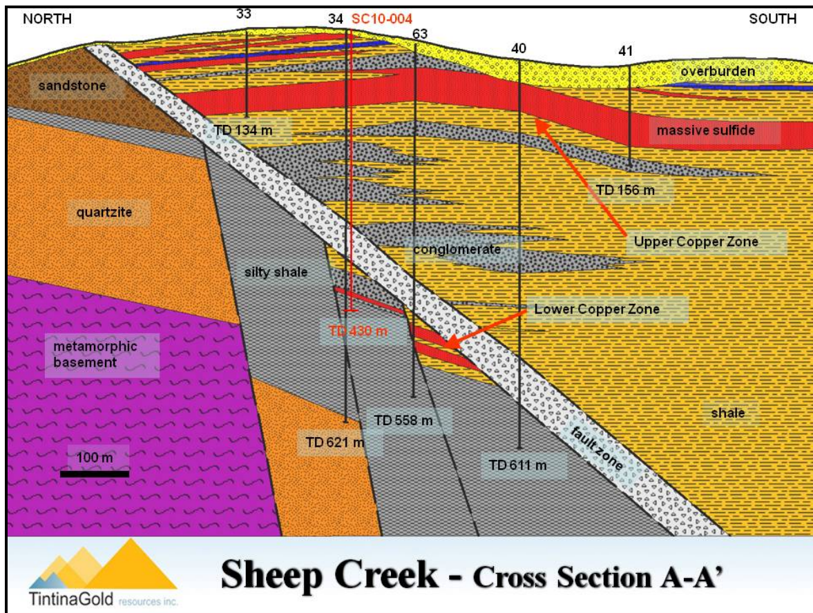
Figure 2 Cross section through historic resource area Sheep Creek, Montana
