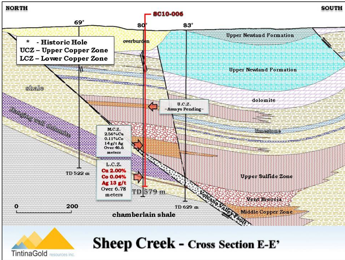
Figure 3 Cross section through Strawberry East area Sheep Creek, Montana
