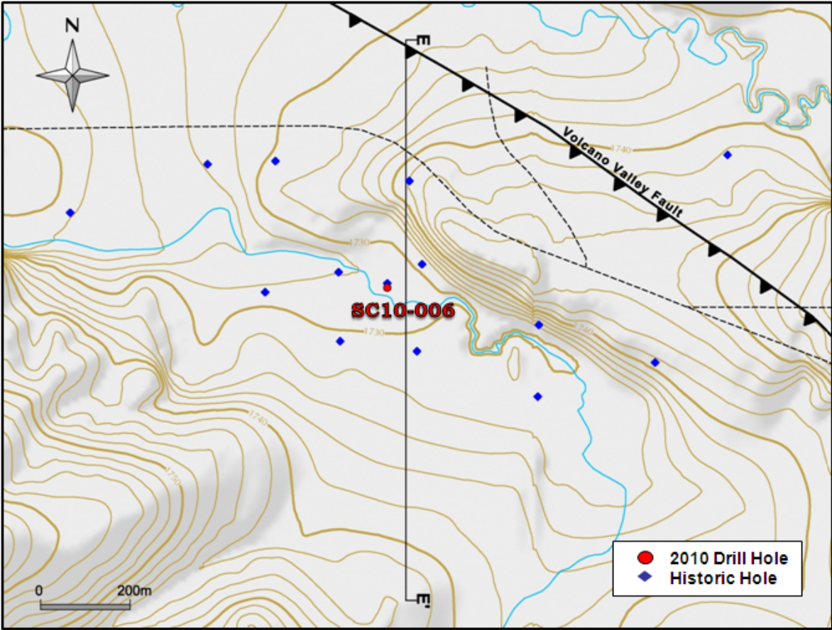
Figure 2 Historic drill pattern and new drilling Strawberry East area, Sheep Creek, Montana
