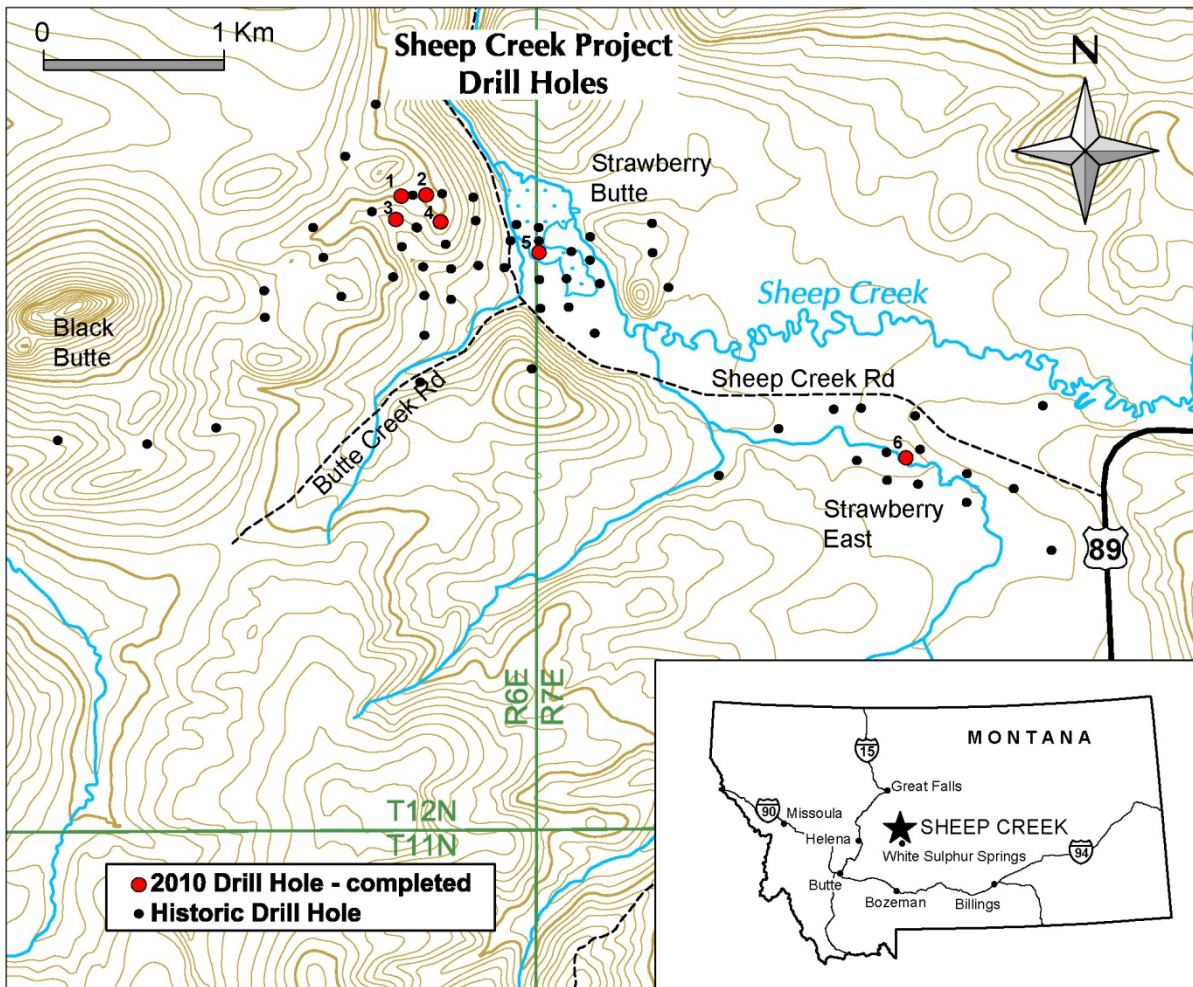
Figure 1 Sheep Creek, Montana
