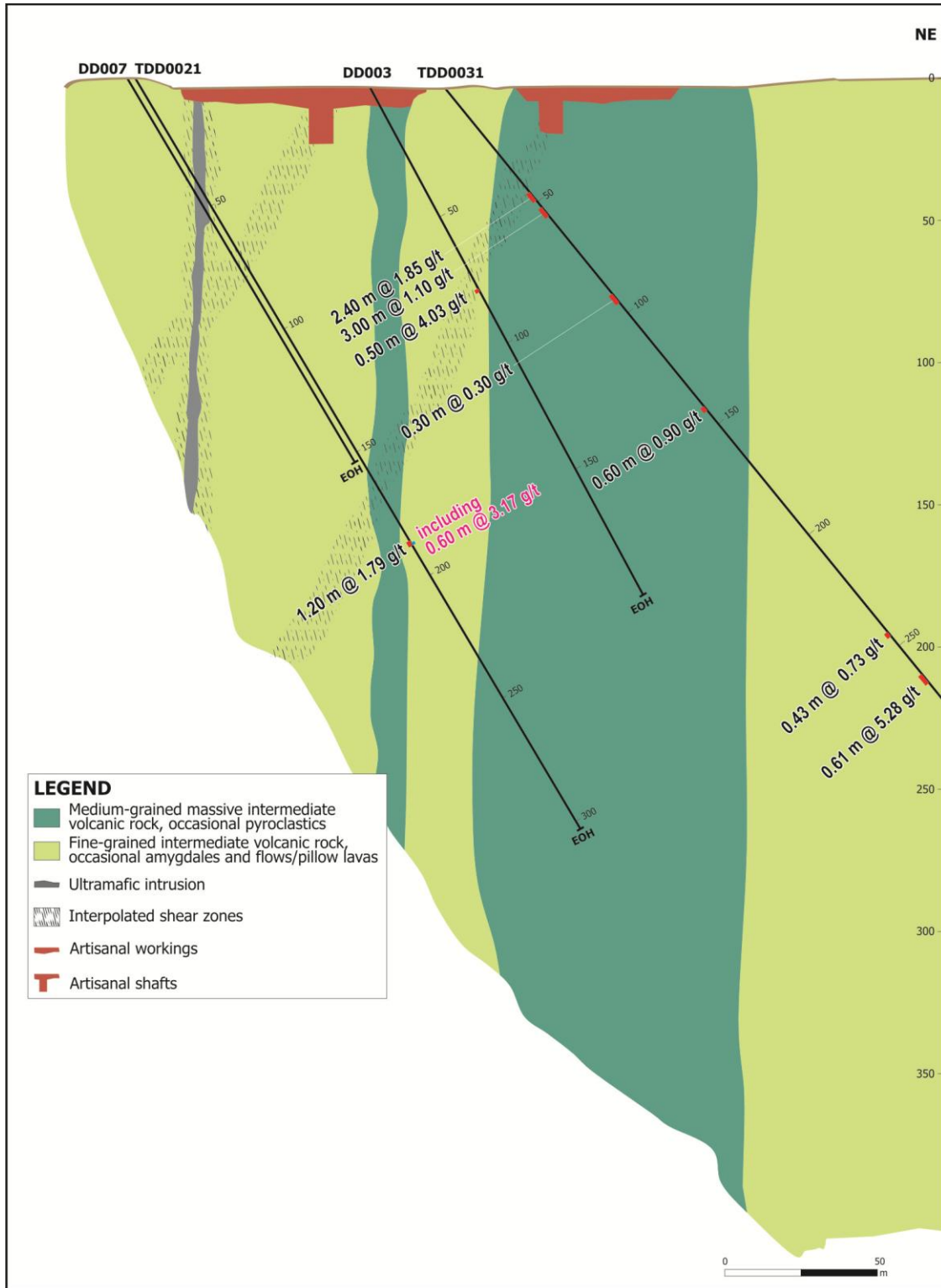
Figure 2: Drill hole Section TDD0021-TDD0031 at Nyakagwe East
