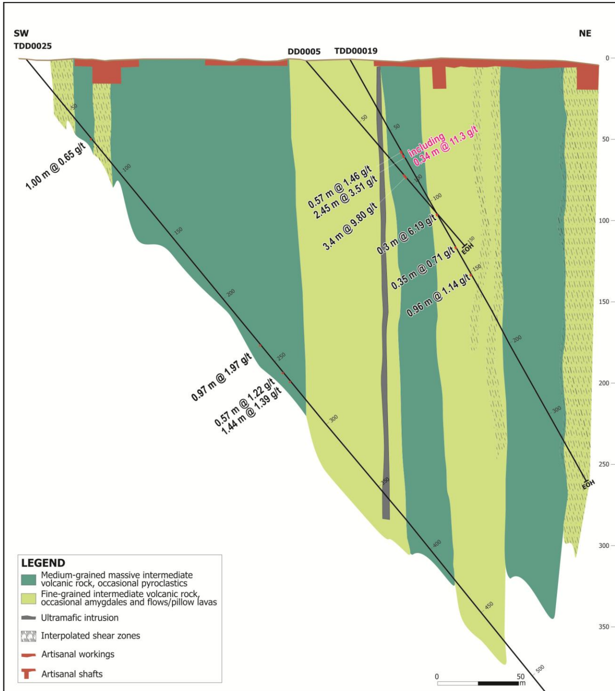
Figure 3: Drill hole Section TDD0025-TDD0019 at Nyakagwe East
