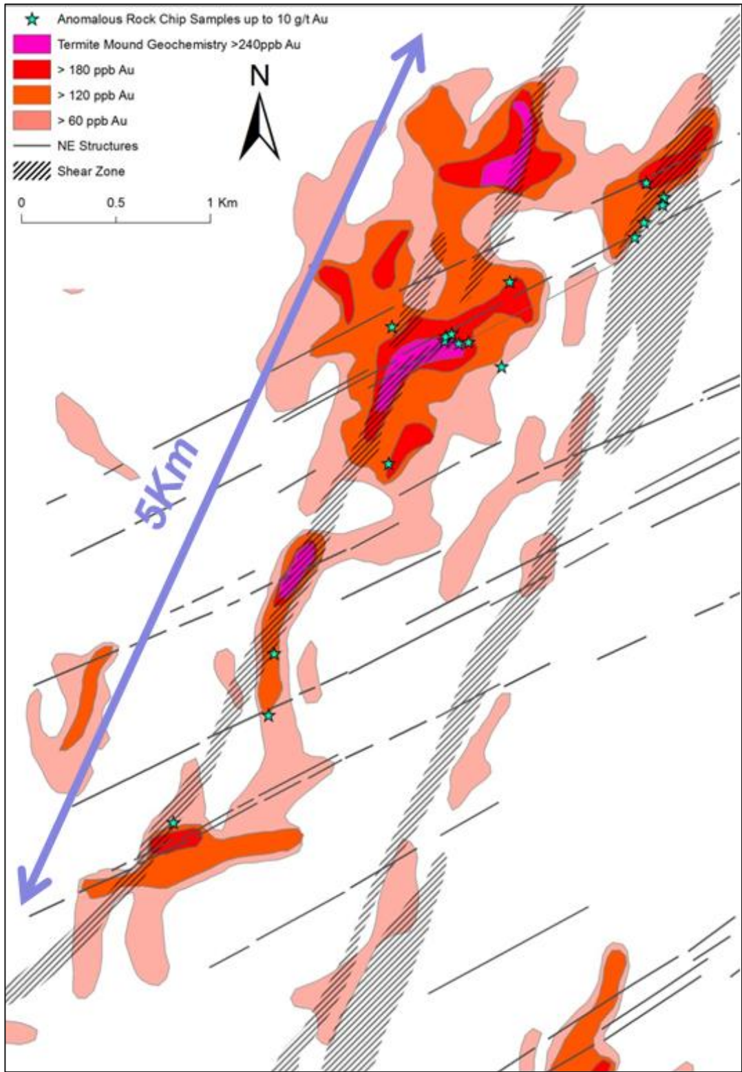
Figure 3: Tourokhoto surface gold geochemistry and structures.
