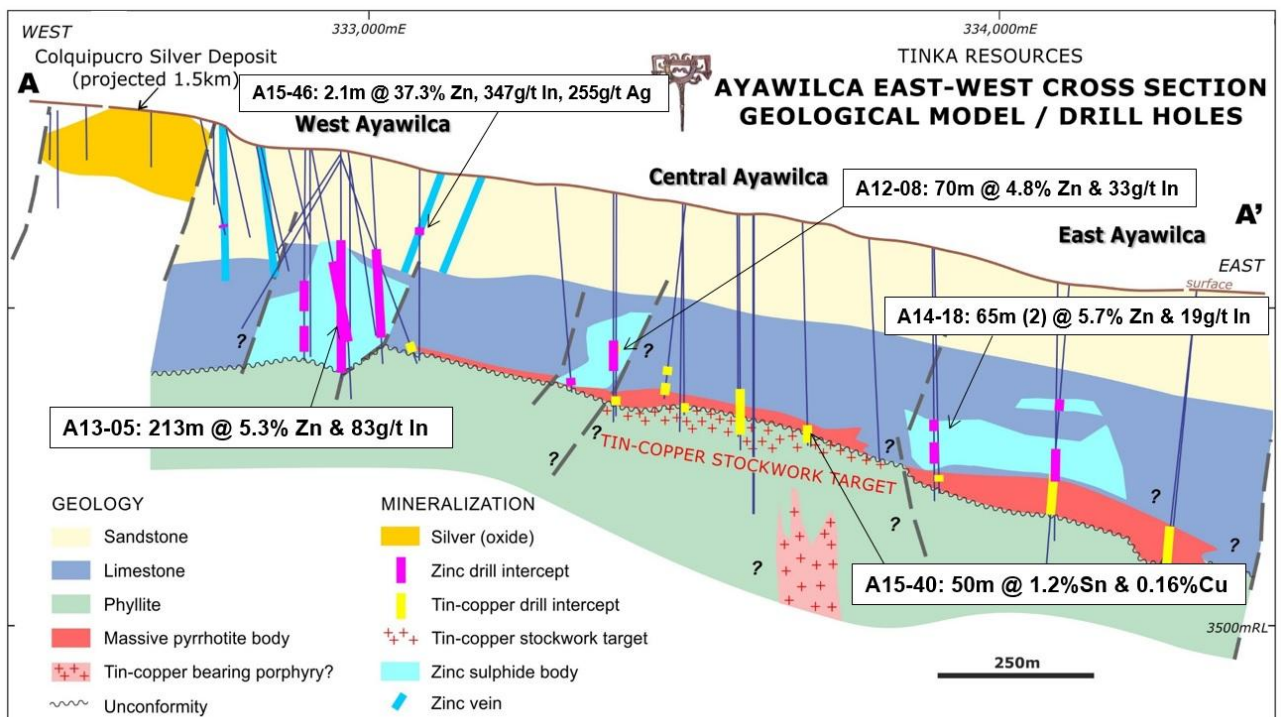
Figure 2. Schematic west-east Geological Section through Ayawilca highlighting selective Zinc and Tin mineralized zones
