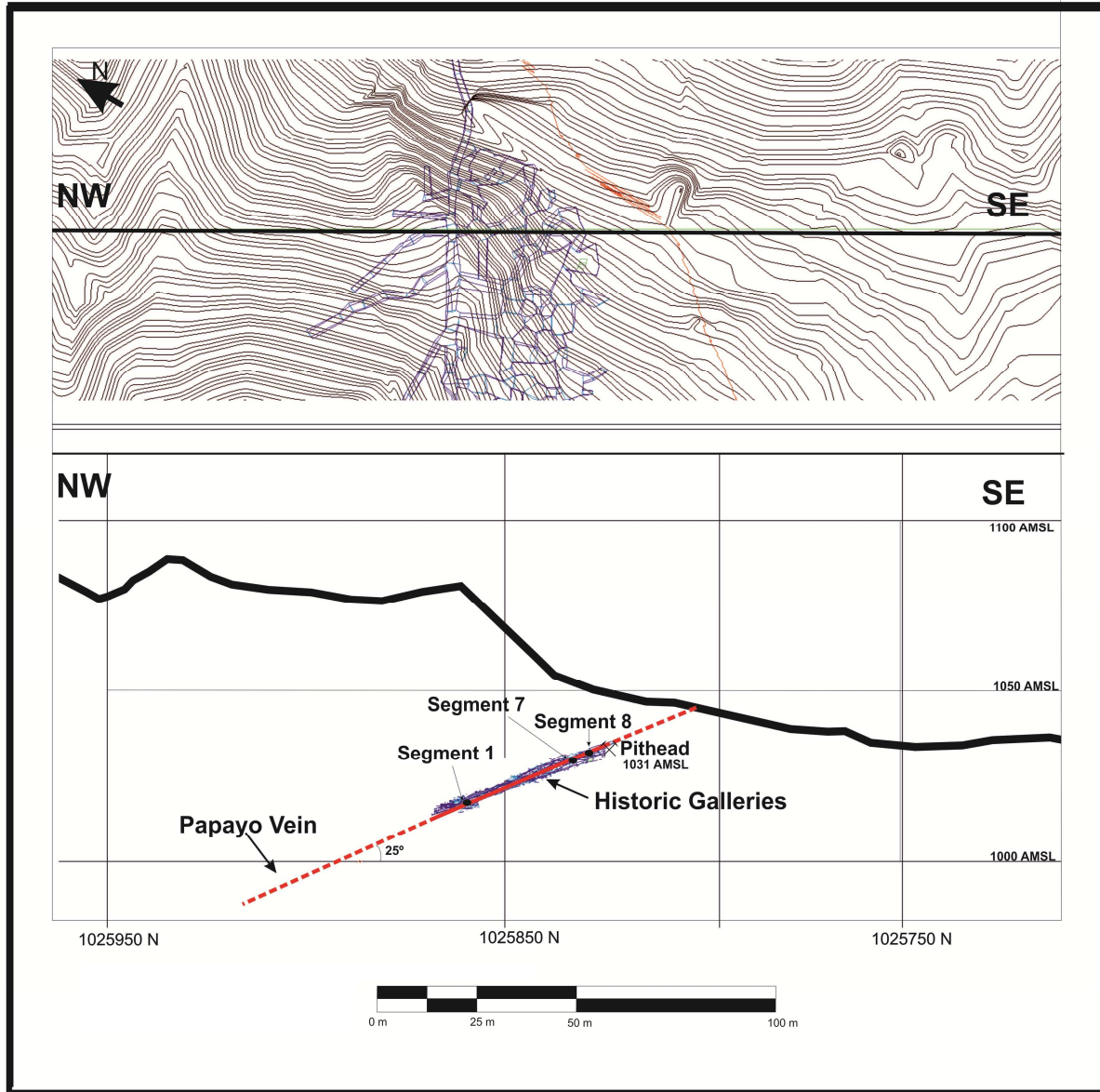
Figure 2. NW-SE Cross section perpendicular to strike of the El Papayo vein, showing its 25° dipping and some significant segments with high gold and silver grades.
