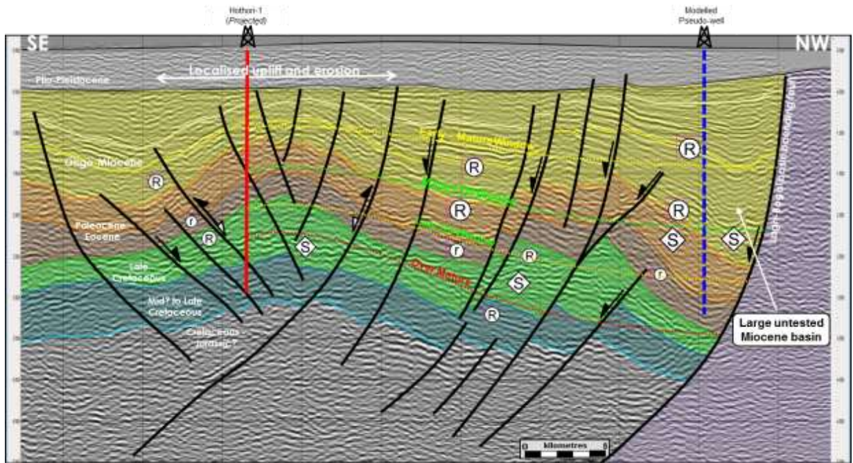
Figure 4 Seismic lines with the results of the 1D geochemical modeling overlain to show that the prospective Miocene Tertiary section is in the oil window on Block 2B.
