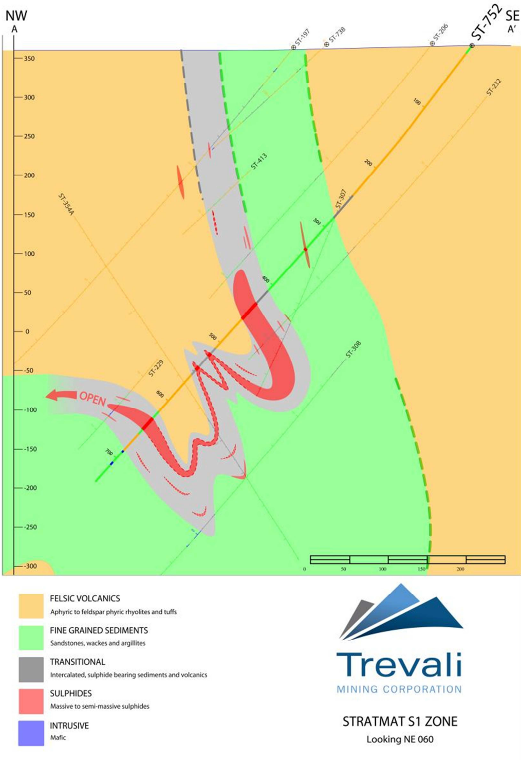
Figure 2: Schematic geological cross-section – Stratmat Deposit, New Brunswick.
