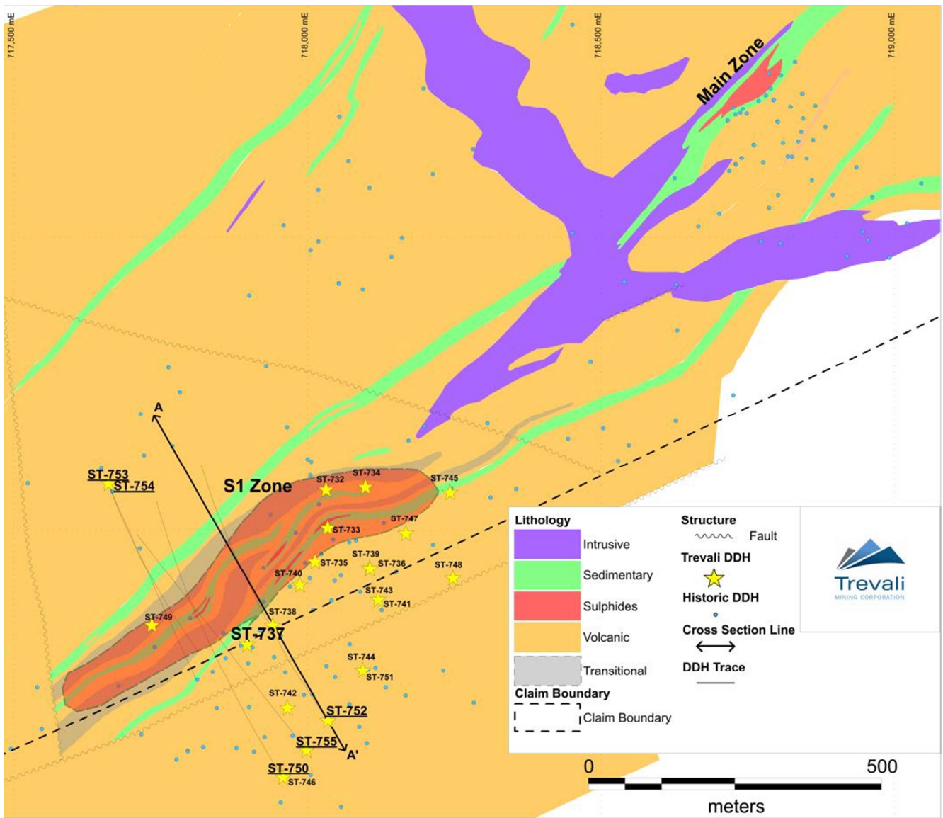
Figure 1: Simplified geological map of a portion of the Stratmat property showing borehole locations.
