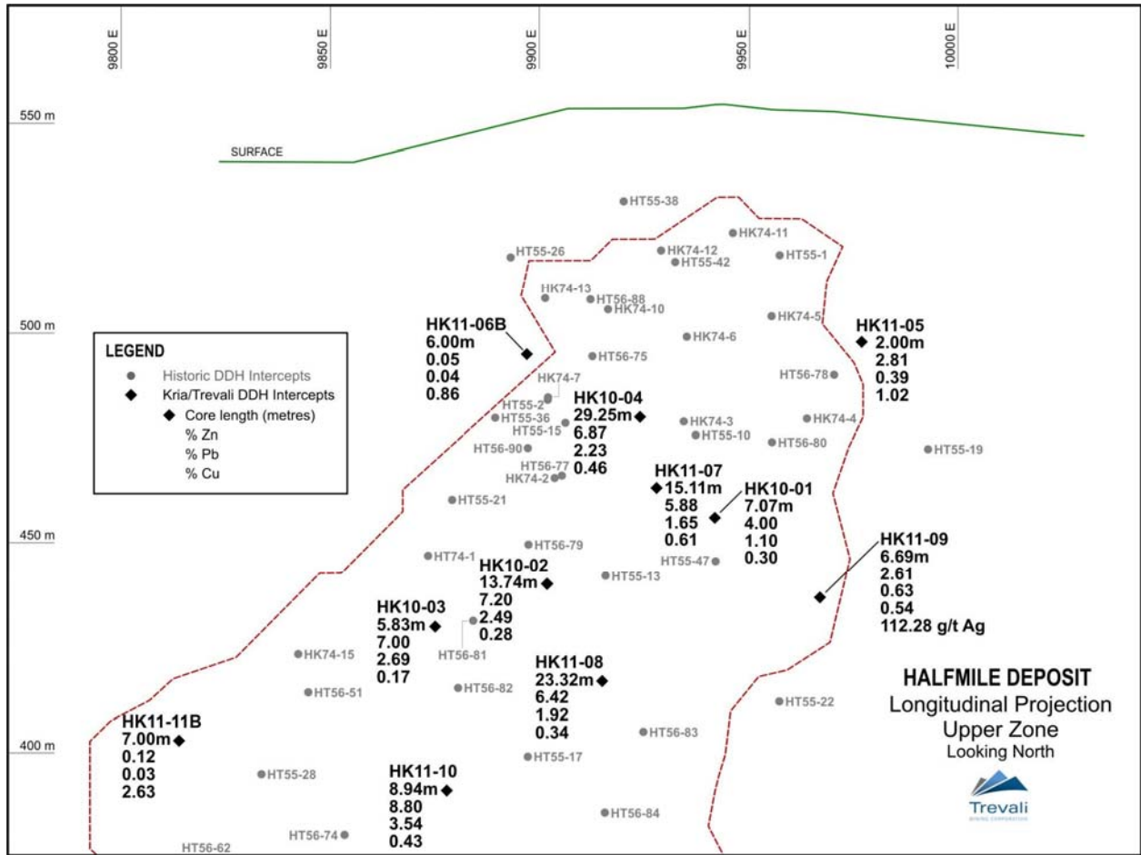
Figure 2 – Longitudinal section of Upper Zone of Halfmile Deposit
