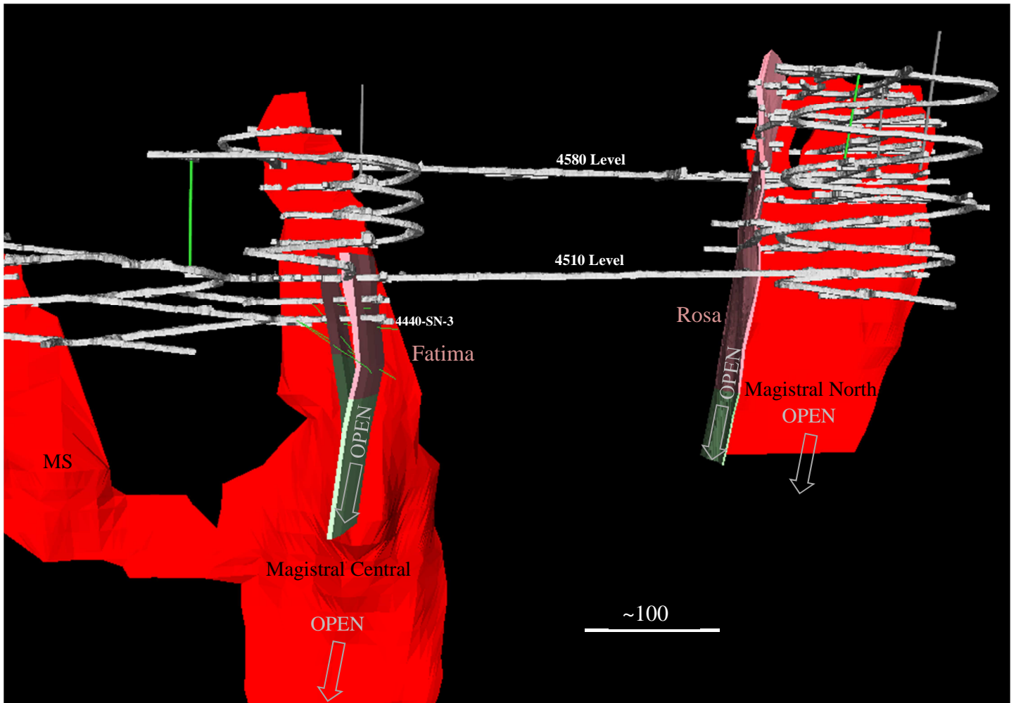
Figure 1: 3D-view looking west showing Magistral North (MN), Magistral Central (MC), partly Magistral South (MS) deposits, Rosa and Fatima zones (illustrative only) with drill holes location at the Santander Mine in Peru.
