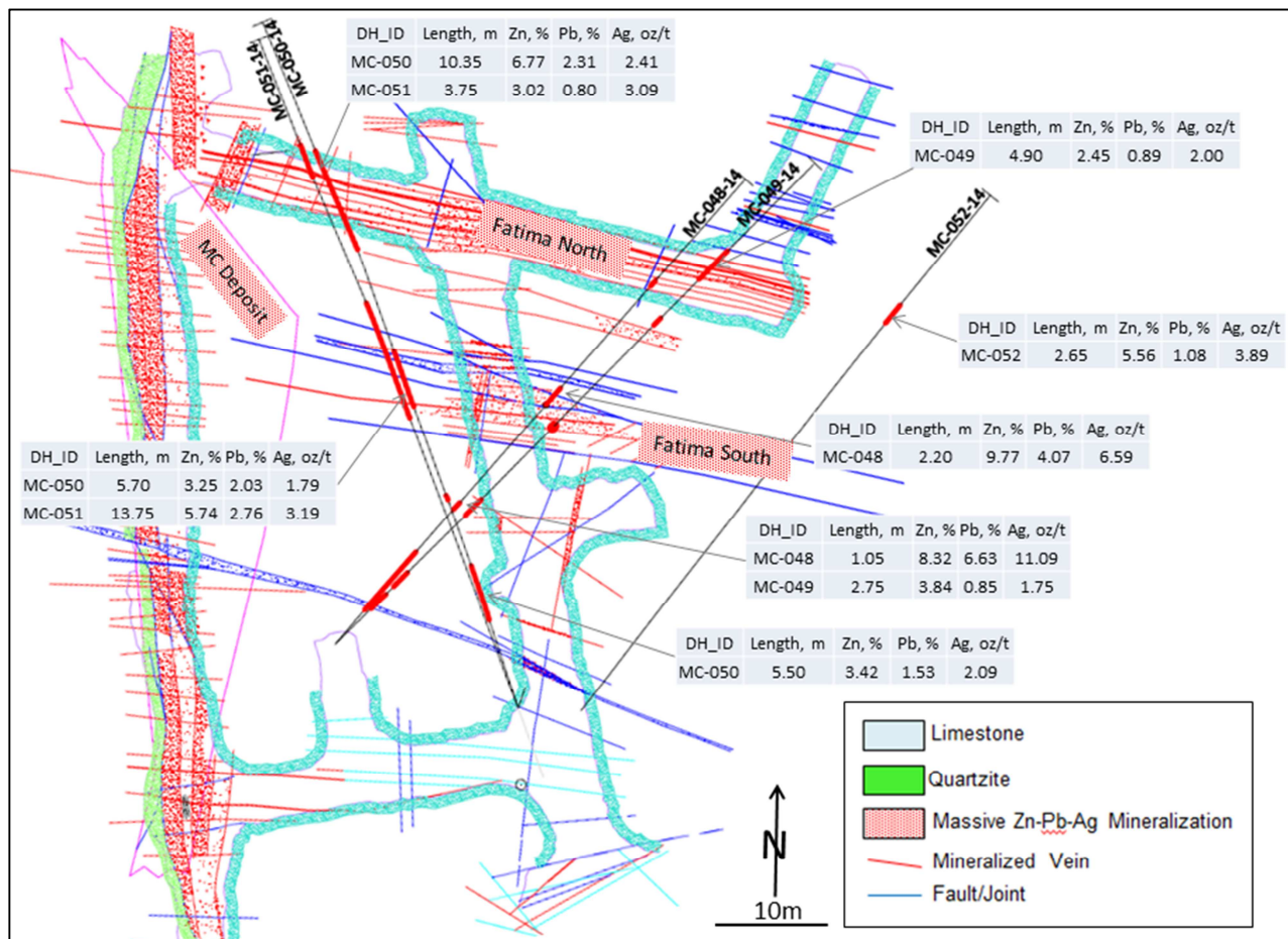
Figure 2: Underground Plan View (Level 4440-SN-3) showing Fatima Zones with drill holes intercepts.
