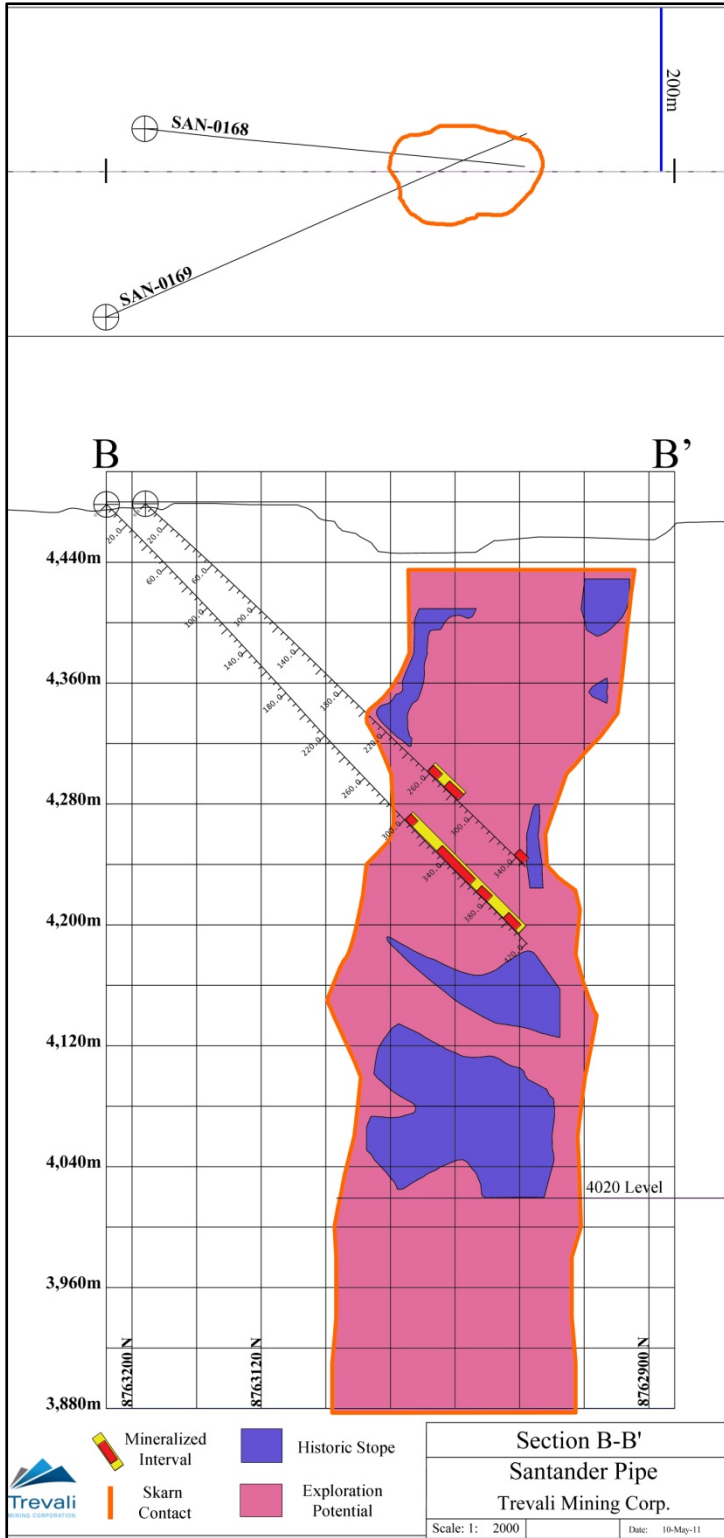
Figure 1 - Drill plan for holes SAN-0168 and 0169 on Santander Pipe
