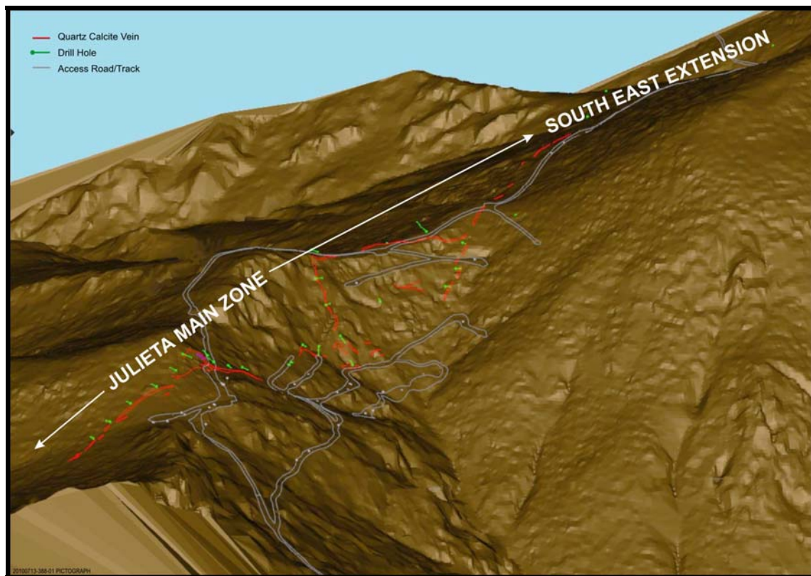
Figure 4: 3D View of the Julieta Main Zone Looking Southeast
