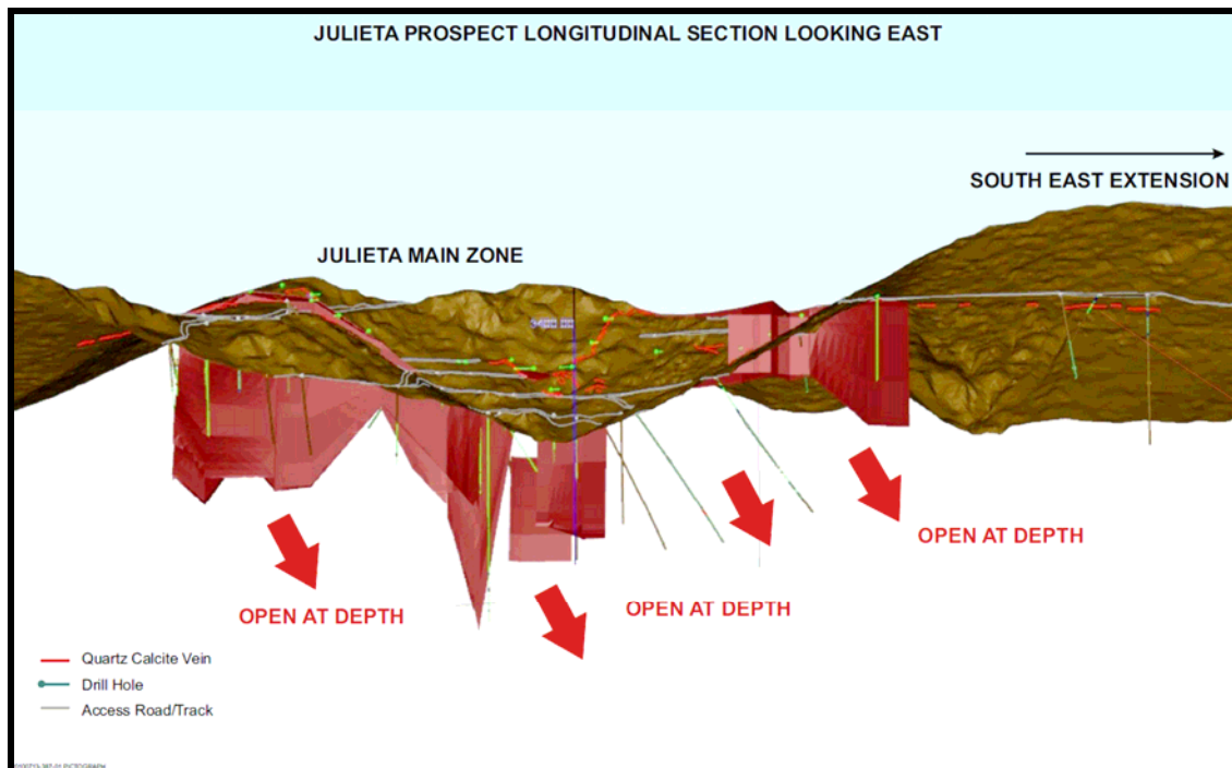
Figure 4: Longitudinal Section through both the Julieta Main Zone and The Southeast Extension Zone
