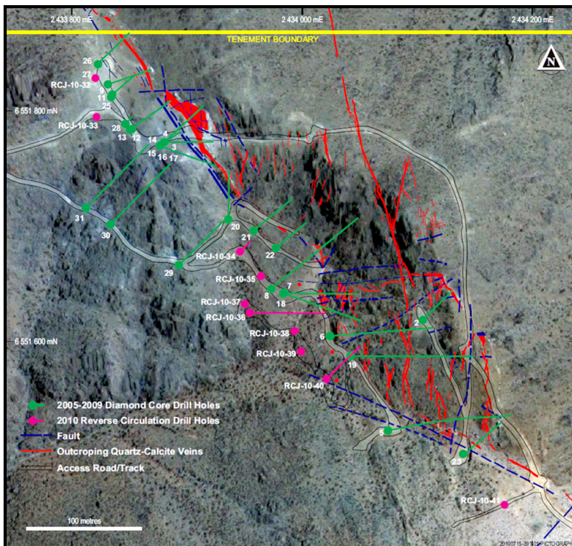
Figure 2: Julieta Main Zone Outcropping Veins on Satellite Image
