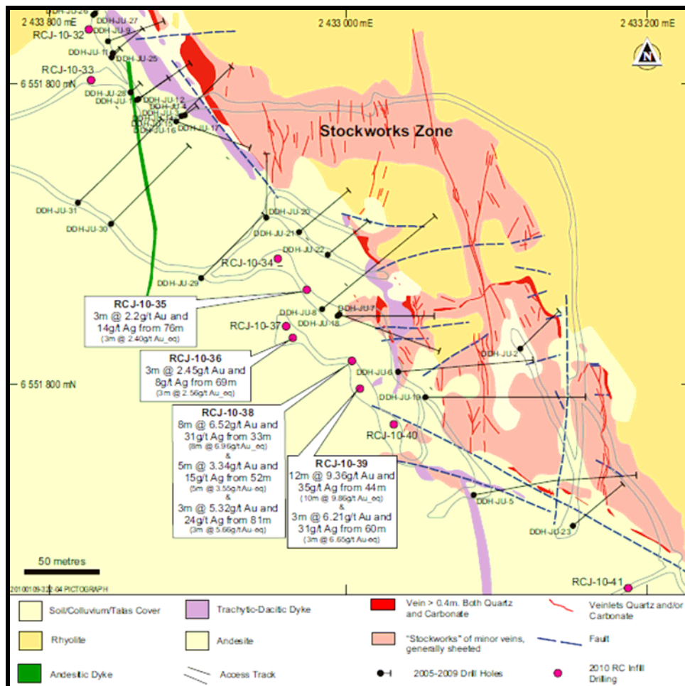
Figure 3: Julieta Main Zone Geology, Drill Collars and Recent RC Intercepts
