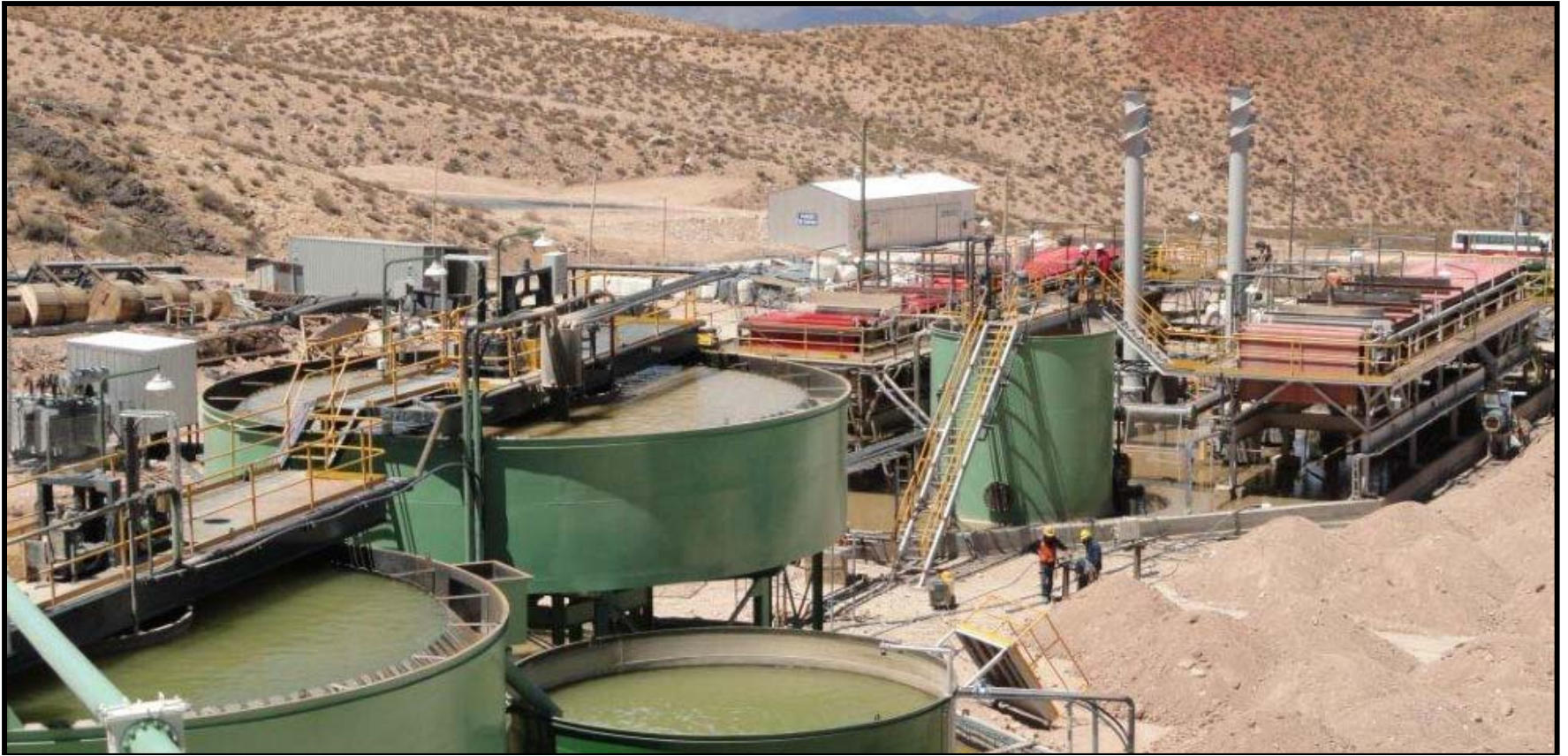
Photo 3: Thickeners and Belt Filters – November 2010
