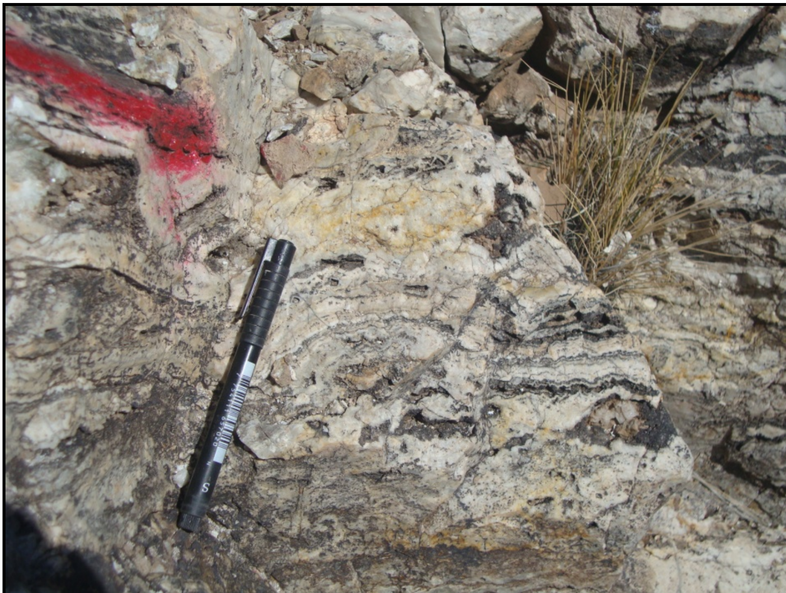
Photo 5: Banded Colloform Texture at Lucia South Vein
