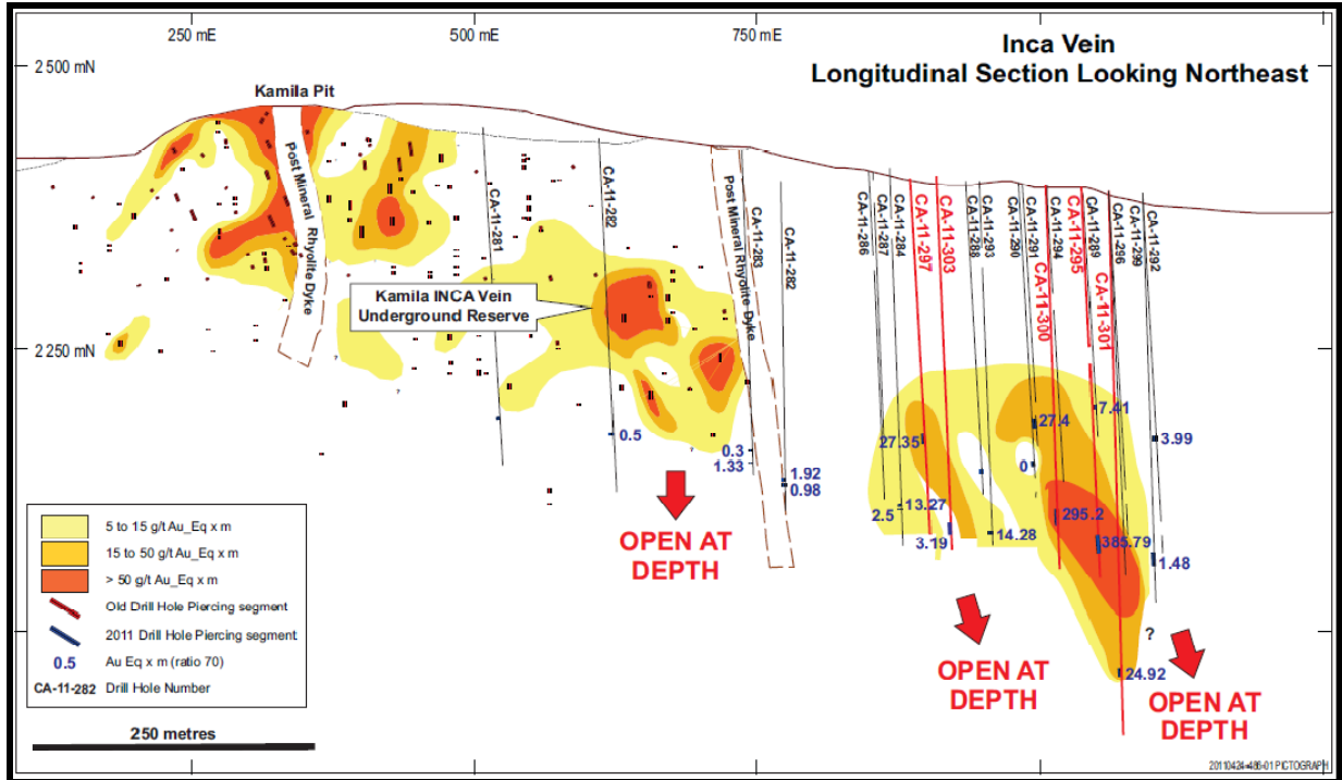
Figure 2: Longitudinal Section Inca Vein (Gold Equivalent gram x metres)
