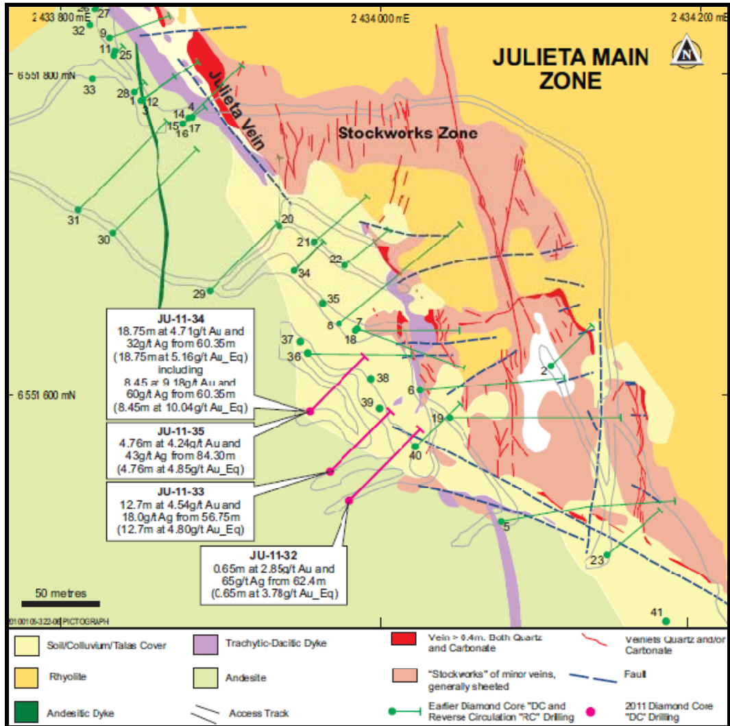
Figure 1: Julieta Main Zone Geology and Drill Collars with Recent Results
