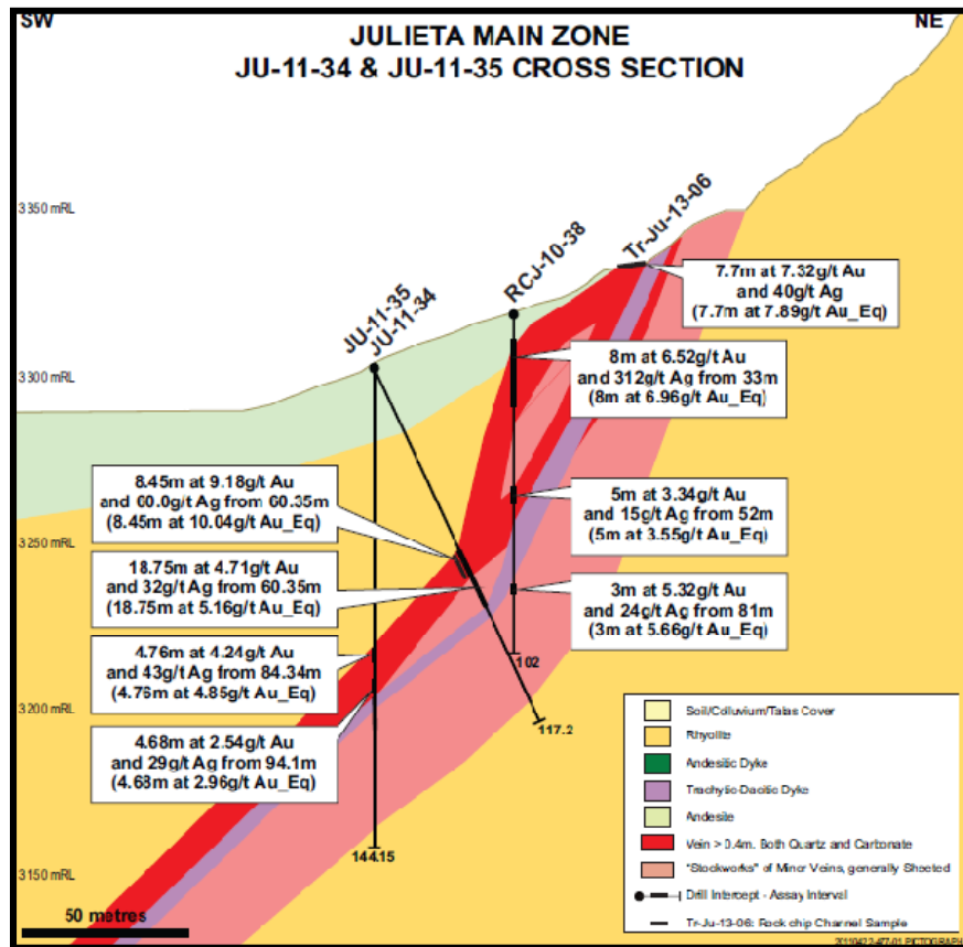
Figure 3: 2011 Drill Cross – Section JU-11-34 and JU-11-35
