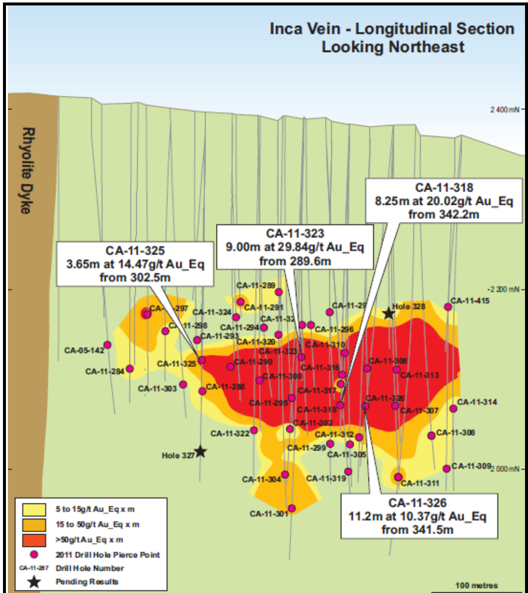
Figure 2: Kamila Southeast Zone – Inca Vein Longitudinal Section
