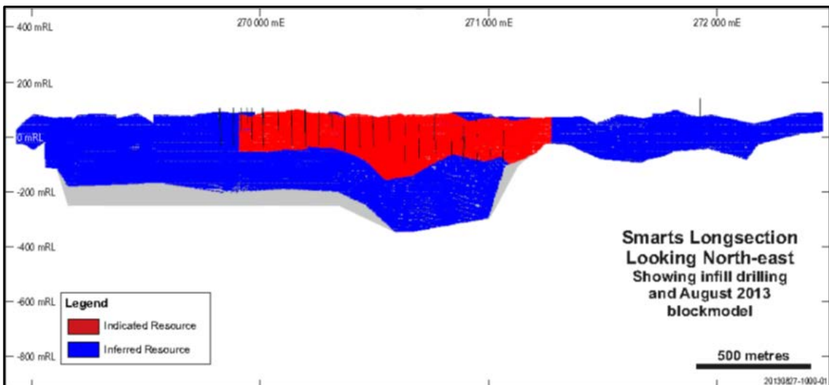
Figure 3: Longitudinal Section showing Block Model Coloured Coded by Resource Category
