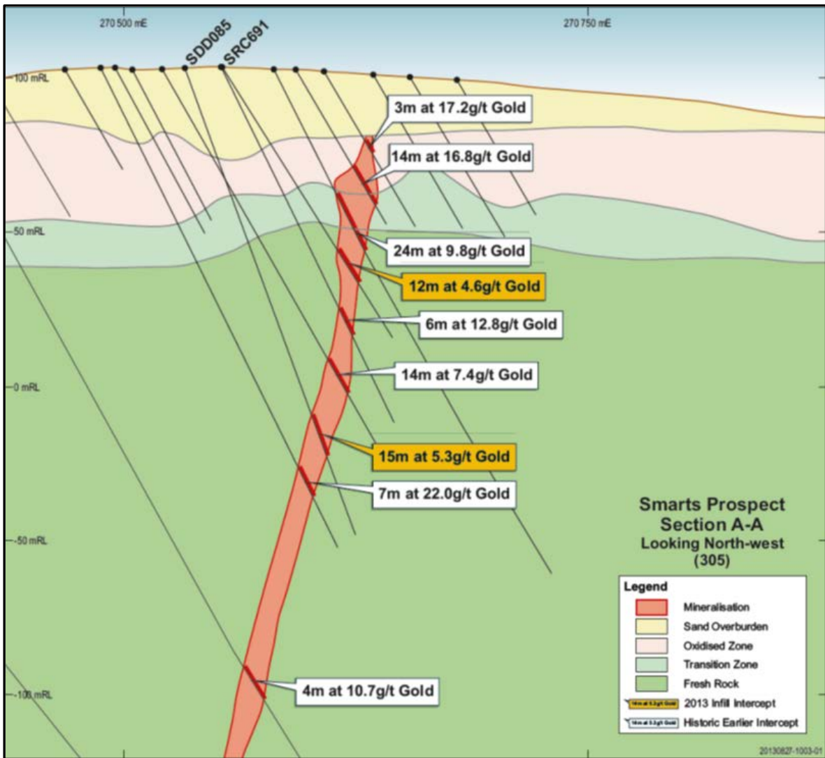
Figure 2: Smarts Zone Cross-Section
