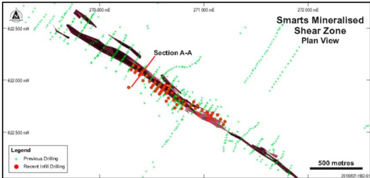
Figure 1: Smarts Deposit Drill Collar Plan
