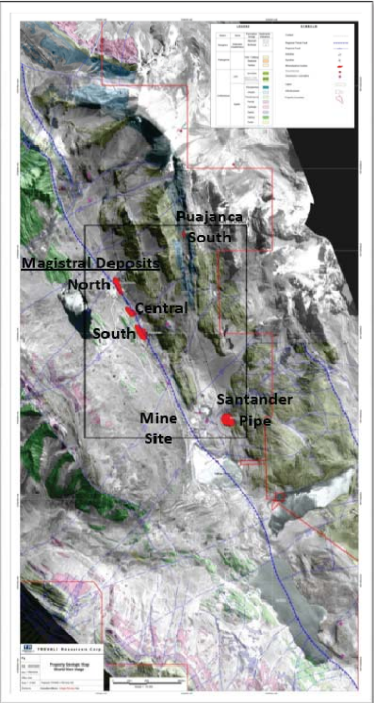
Figure 2: Trevali's 44km 2 Santander silver-lead-zinc mine project in west-central Peru.
