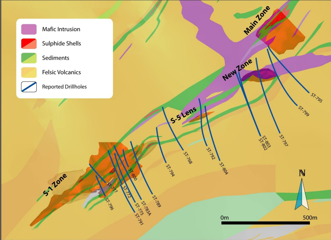
Figure 1: Geology map with 3-D projection of mineralization.
