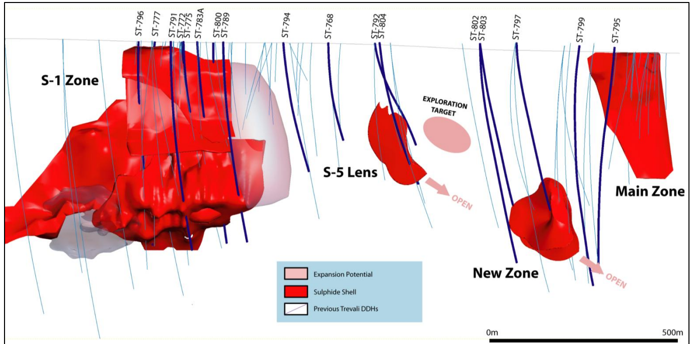
Figure 2: 3D longitudinal section view of the Stratmat Deposits looking N330°
